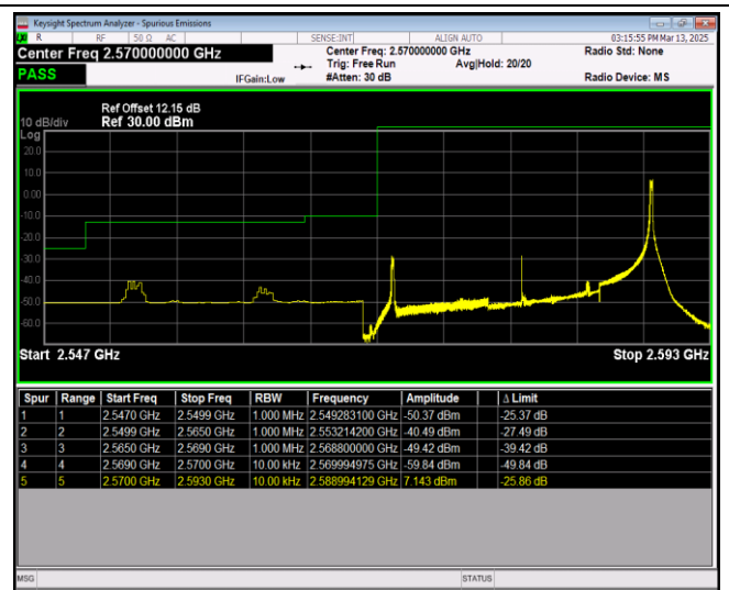
Band38-20MHz-16QAM-38150-1RB#0
