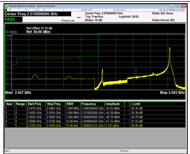
Band38-20MHz-64QAM-38150-1RB#0
