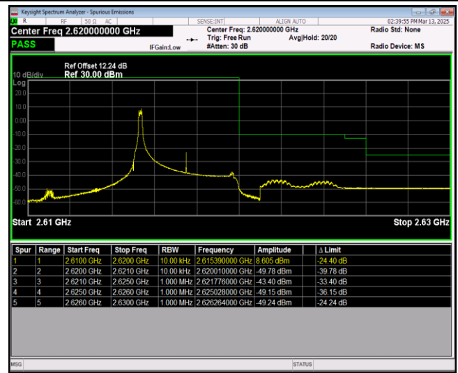
Band38-5MHz-16QAM-38225-25RB#0
