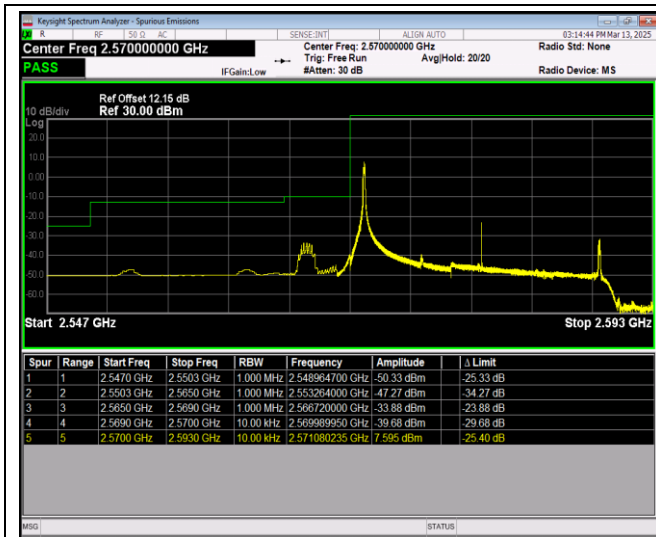
Band38-20MHz-QPSK-37850-100RB#0
