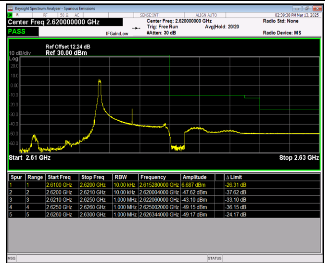
Band38-5MHz-QPSK-38225-25RB#0
