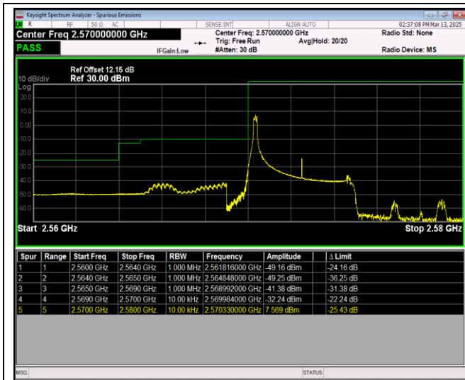
Band38-5MHz-16QAM-37775-25RB#0
