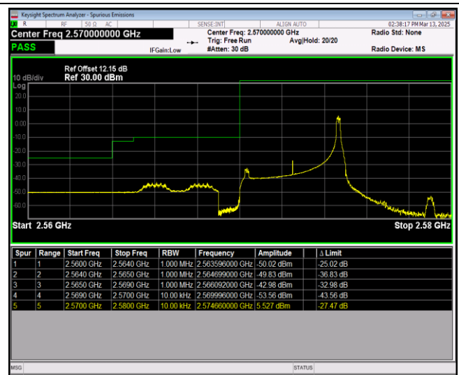
Band38-5MHz-64QAM-38225-1RB#0
