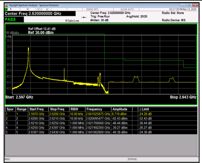
Band38-20MHz-QPSK-38150-100RB#0
