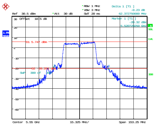
802.11n40_5550MHz
