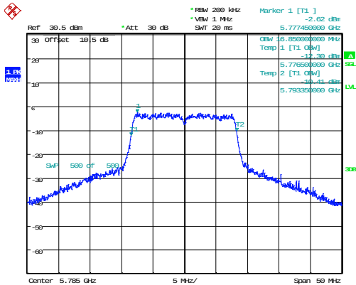
802.11a_5785MHz
