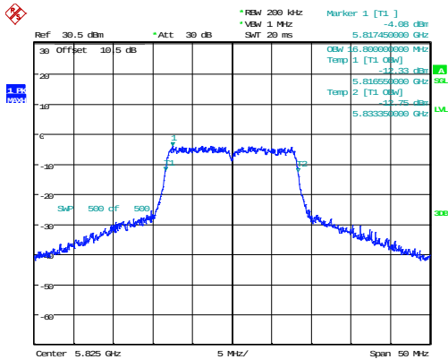
802.11a_5825MHz
