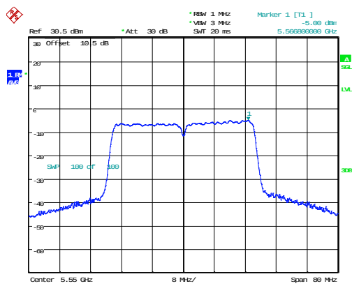
802.11n40_5550MHz
