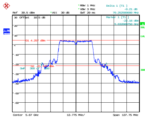
802.11n40_5670MHz
