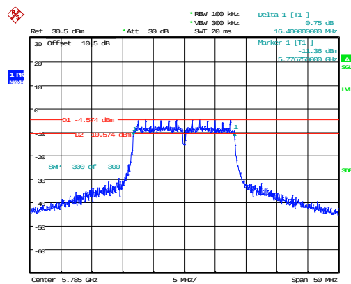
802.11a_5785MHz
