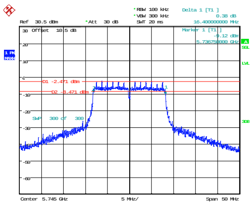
802.11a_5745MHz
