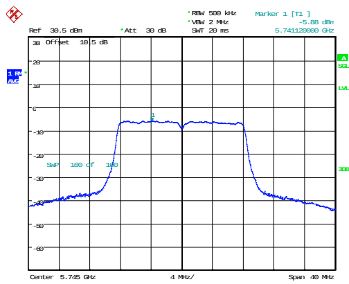
802.11a_5745MHz
