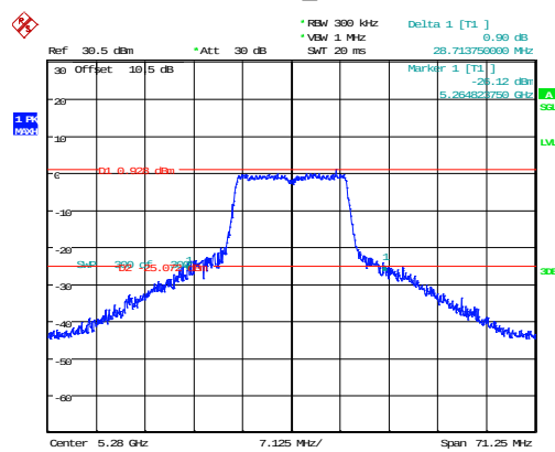
802.11a_5280MHz
