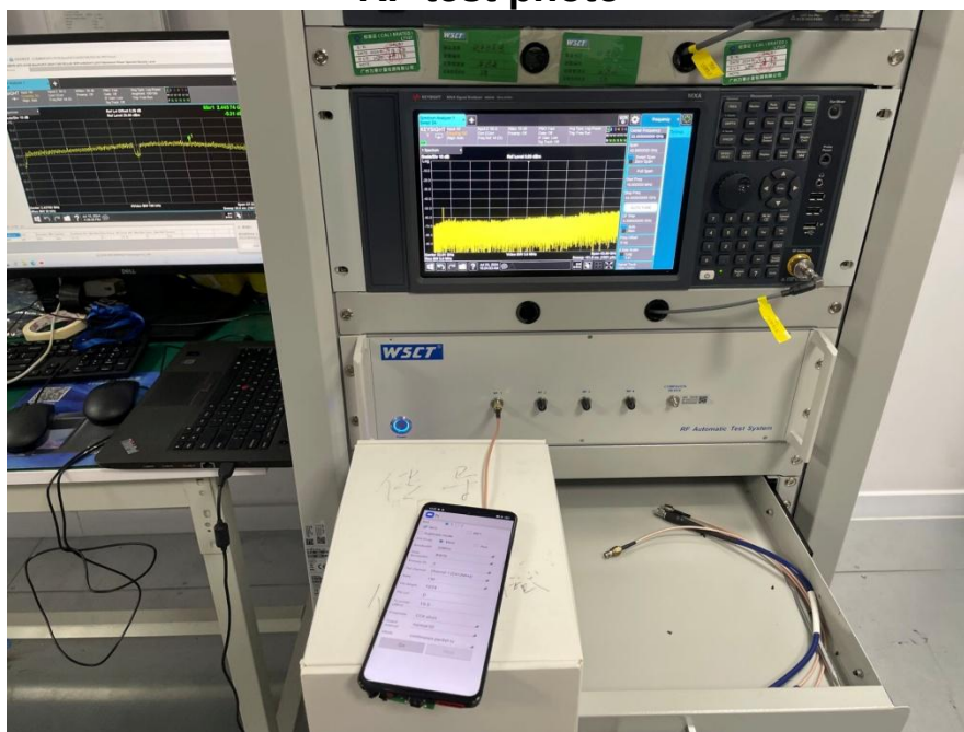
RF test photo
