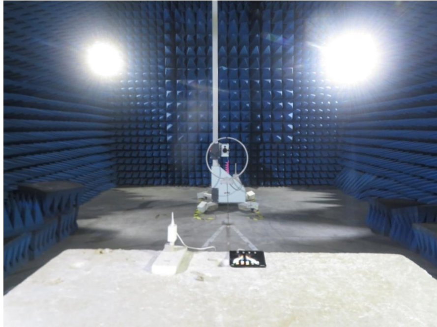
RADIATED EMISSION TEST BELOW 30MHz
