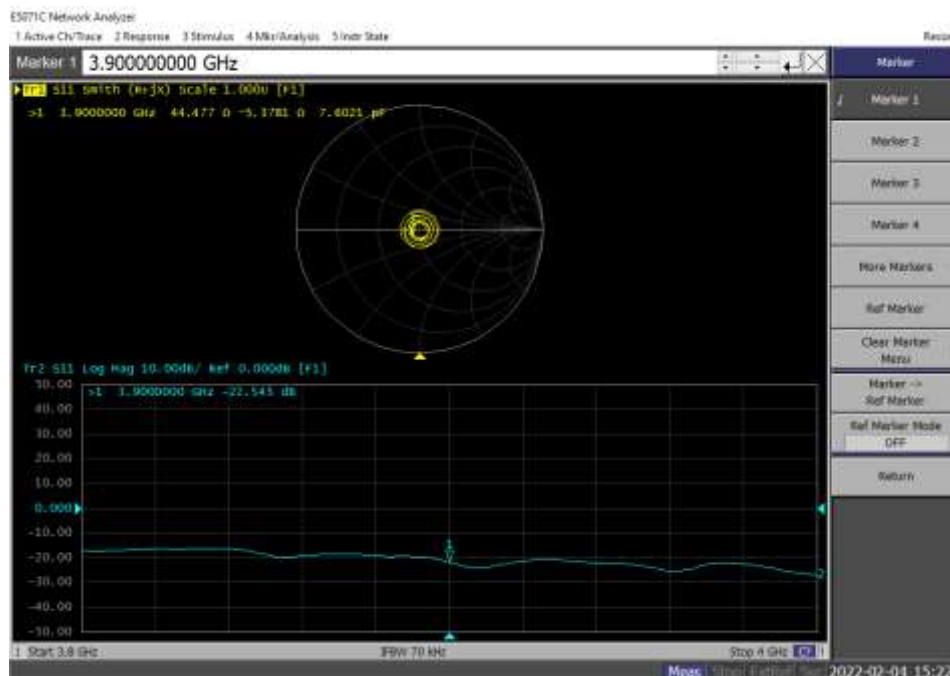
Measurement Plot for Head TSL In 2022
