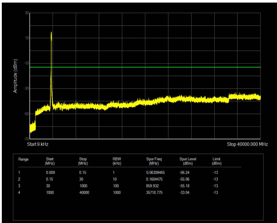
n77(3700-3980) SCS=30kHz DFT_QPSK BW=10MHz Channel=665000 RB=1@23
