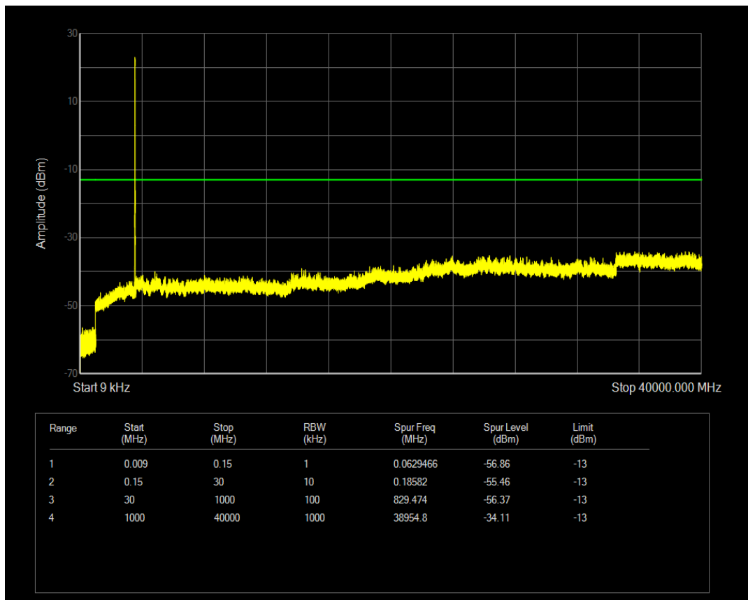
n77(3450-3550) SCS=30kHz DFT_QPSK BW=10MHz Channel=636332 RB=1@0
