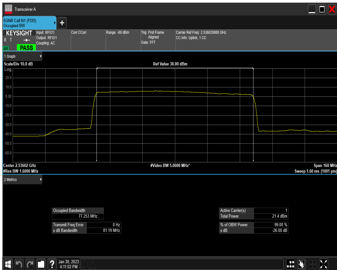
n41 SCS=30kHz CP_QPSK BW=80MHz Channel=507204 RB=217@0
