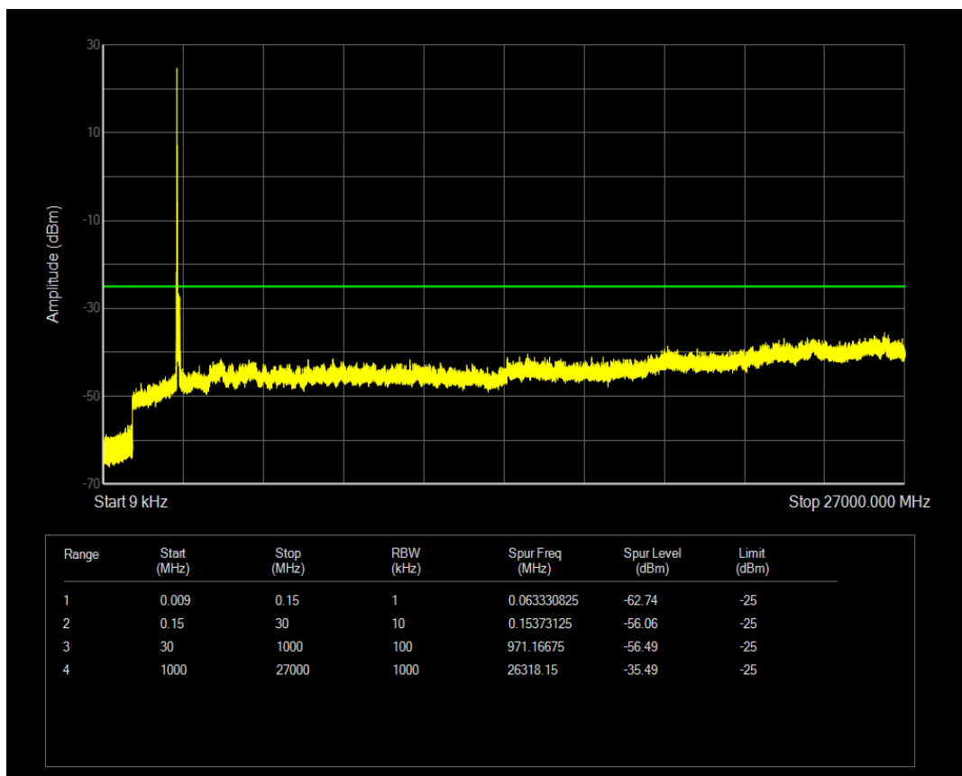
n41 SCS=30kHz DFT_QPSK BW=100MHz Channel=509202 RB=1@272
