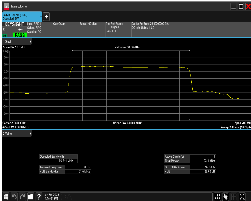
n41 SCS=30kHz DFT_QAM256 BW=100MHz Channel=528000 RB=270@0
