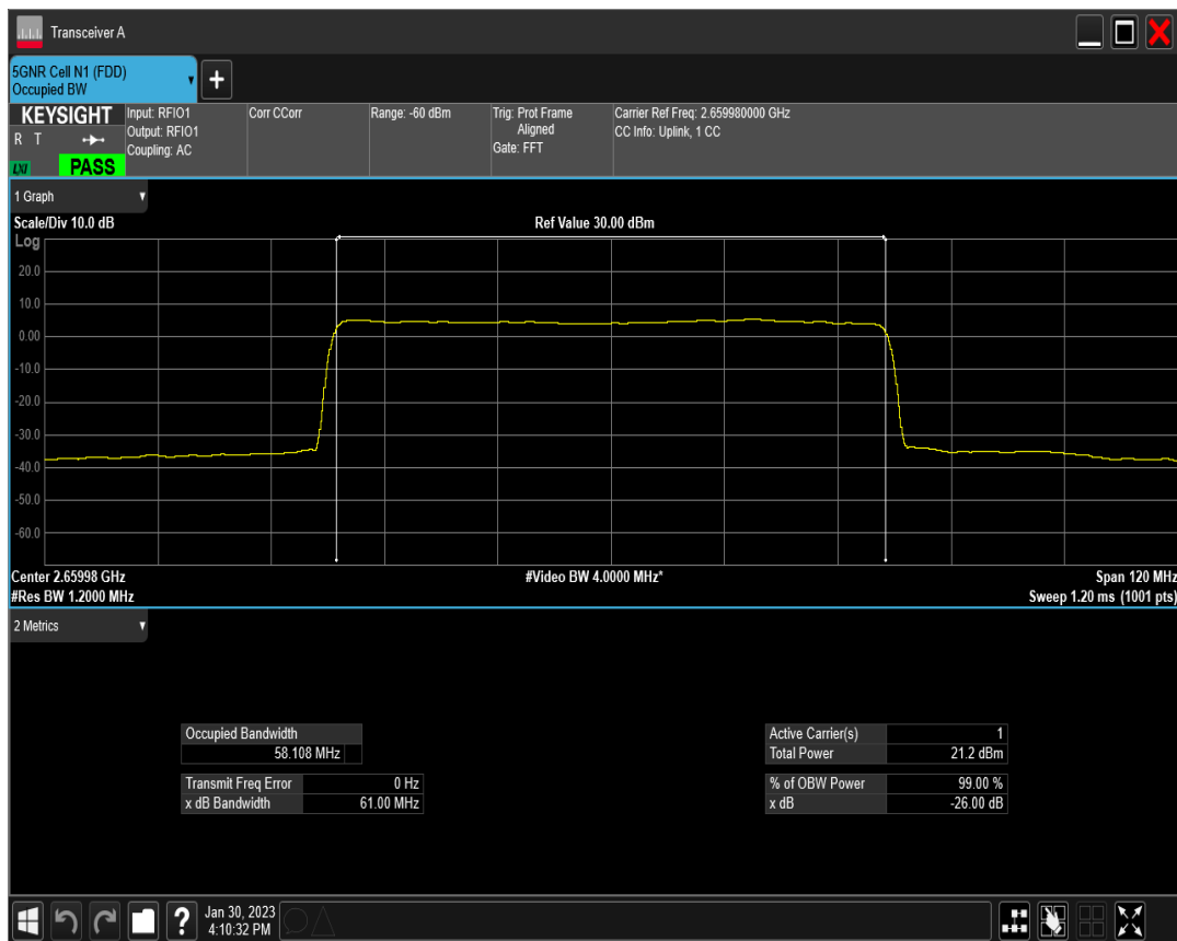
n41 SCS=30kHz CP_QPSK BW=60MHz Channel=531996 RB=162@0
