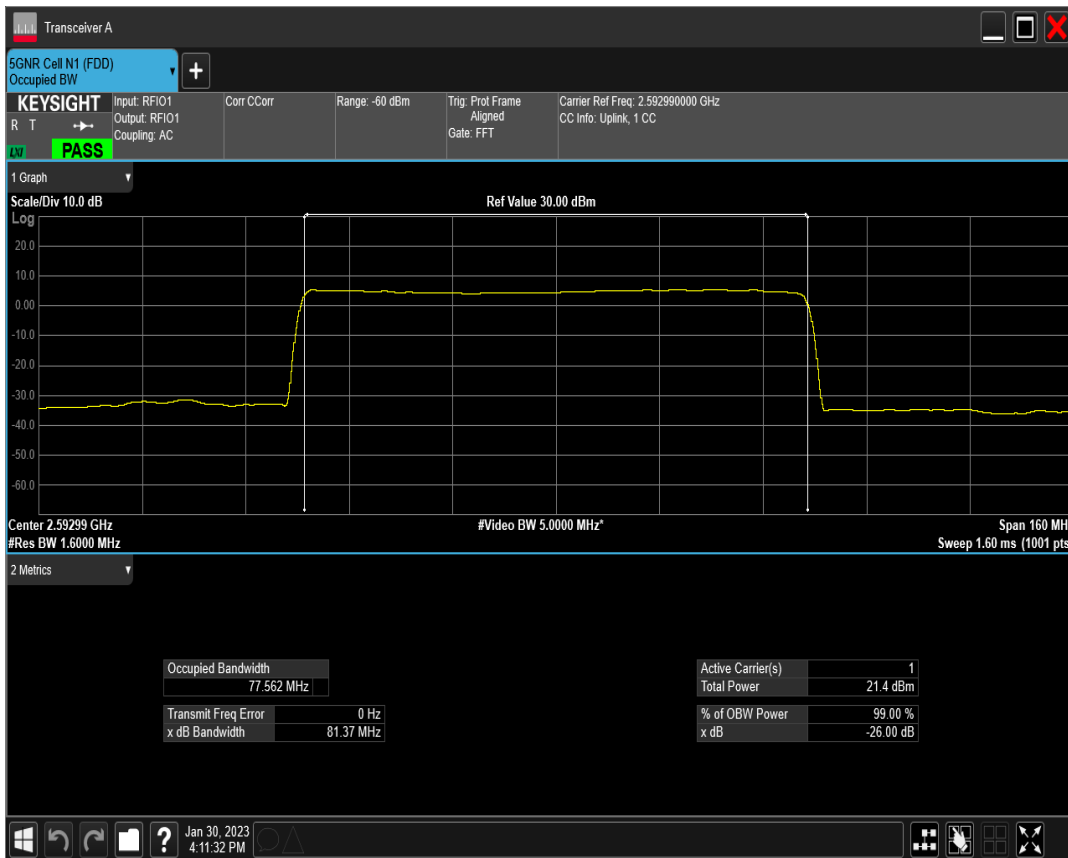
n41 SCS=30kHz CP_QPSK BW=80MHz Channel=518598 RB=217@0
