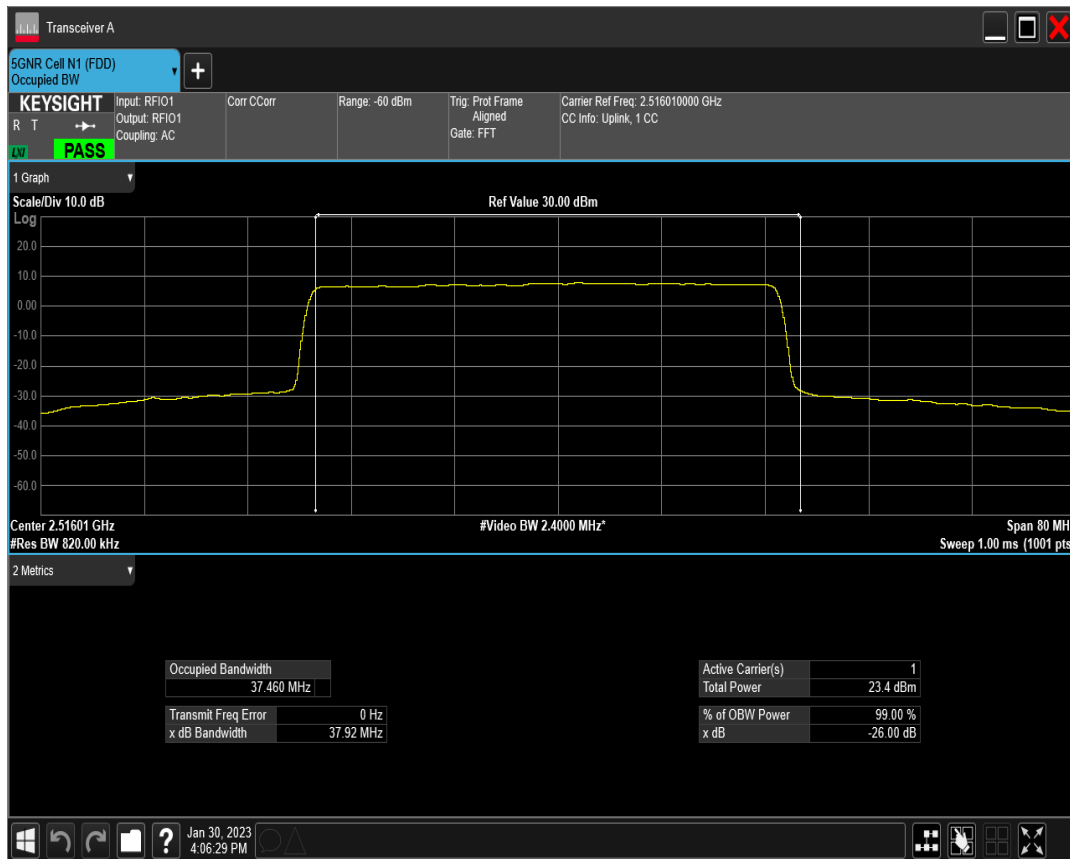
n41 SCS=30kHz DFT_QAM256 BW=40MHz Channel=503202 RB=100@0
