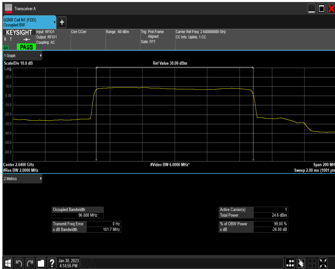
n41 SCS=30kHz DFT_QAM16 BW=100MHz Channel=528000 RB=270@0
