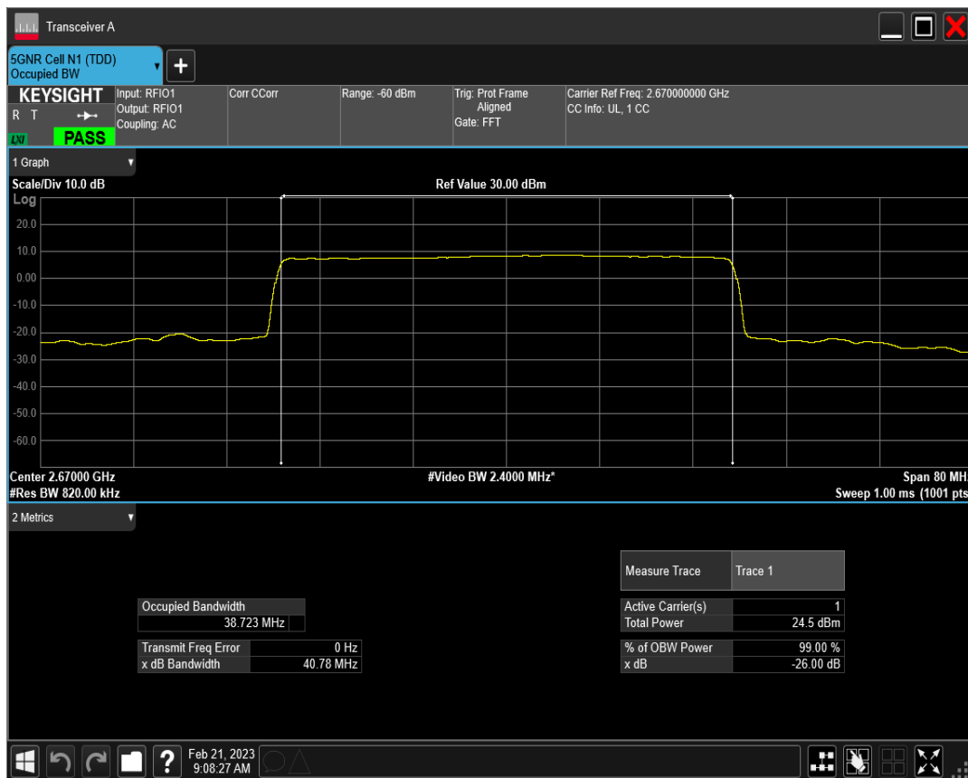
n41 SCS=15kHz DFT_QAM16 BW=40MHz Channel=534000 RB=216@0
