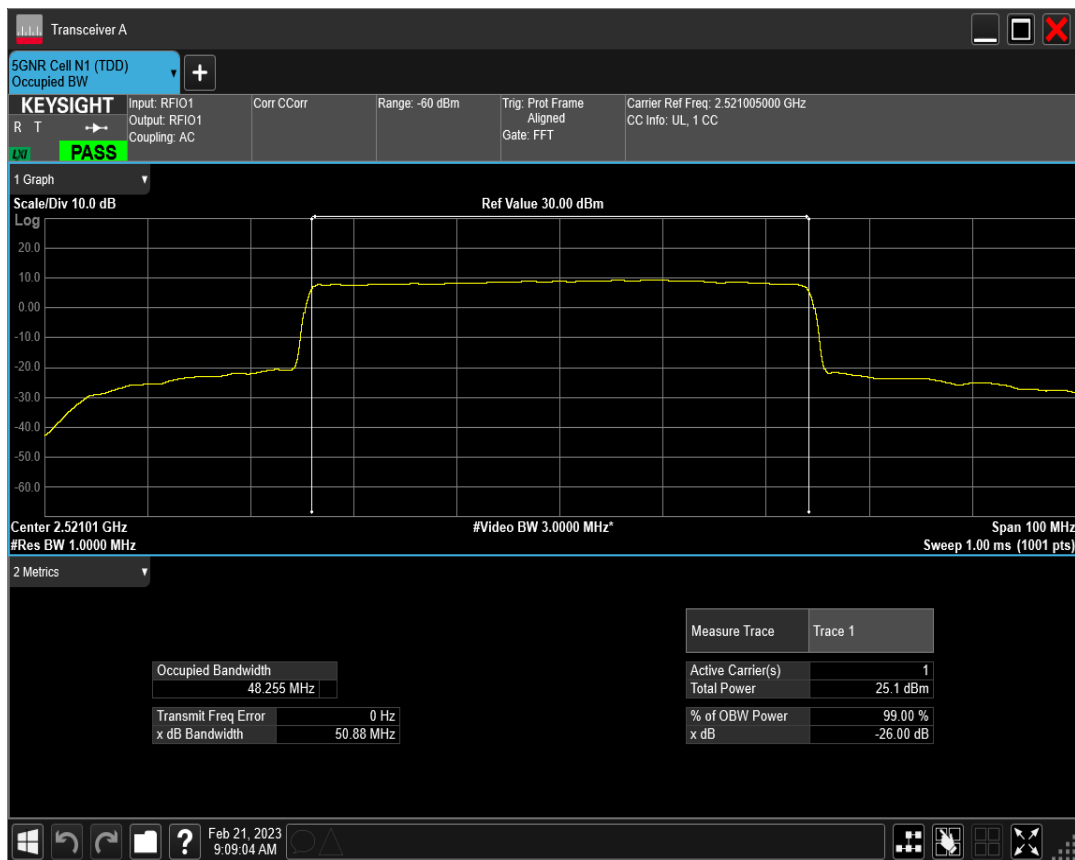
n41 SCS=15kHz DFT_QAM16 BW=50MHz Channel=504201 RB=270@0
