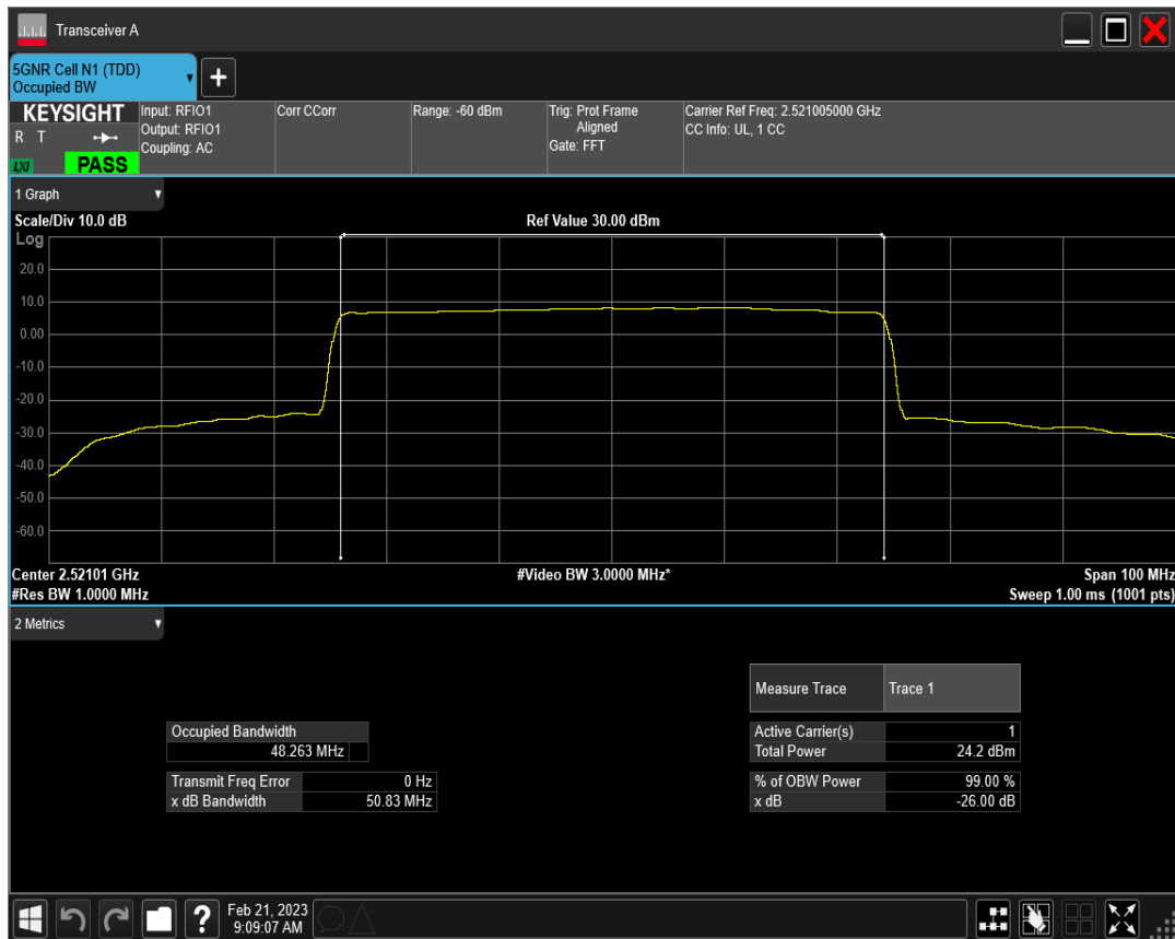
n41 SCS=15kHz DFT_QAM64 BW=50MHz Channel=504201 RB=270@0
