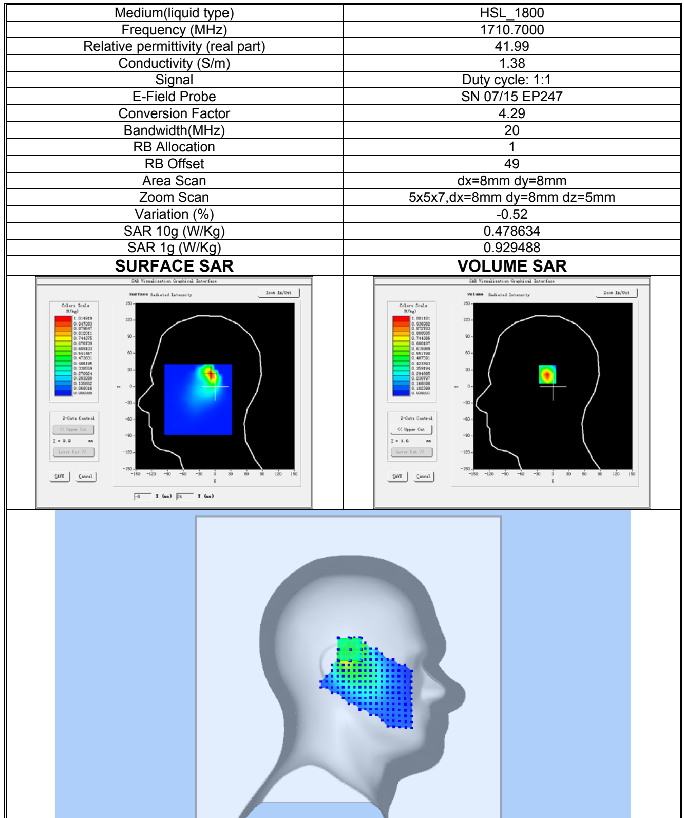
Plot 13:LTE BAND 4, Low channel (Left Head Tilt) Product Description:Mobile Phone Test Date: 2020-01-10
