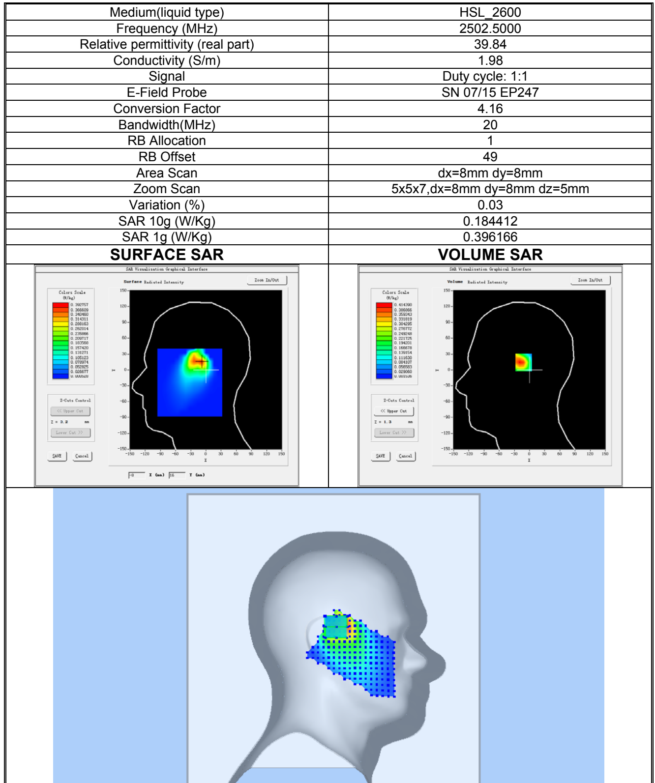
Plot 17:LTE BAND 7, Low channel (Left Head Tilt) Product Description: Mobile Phone Test Date: 2020-01-10
