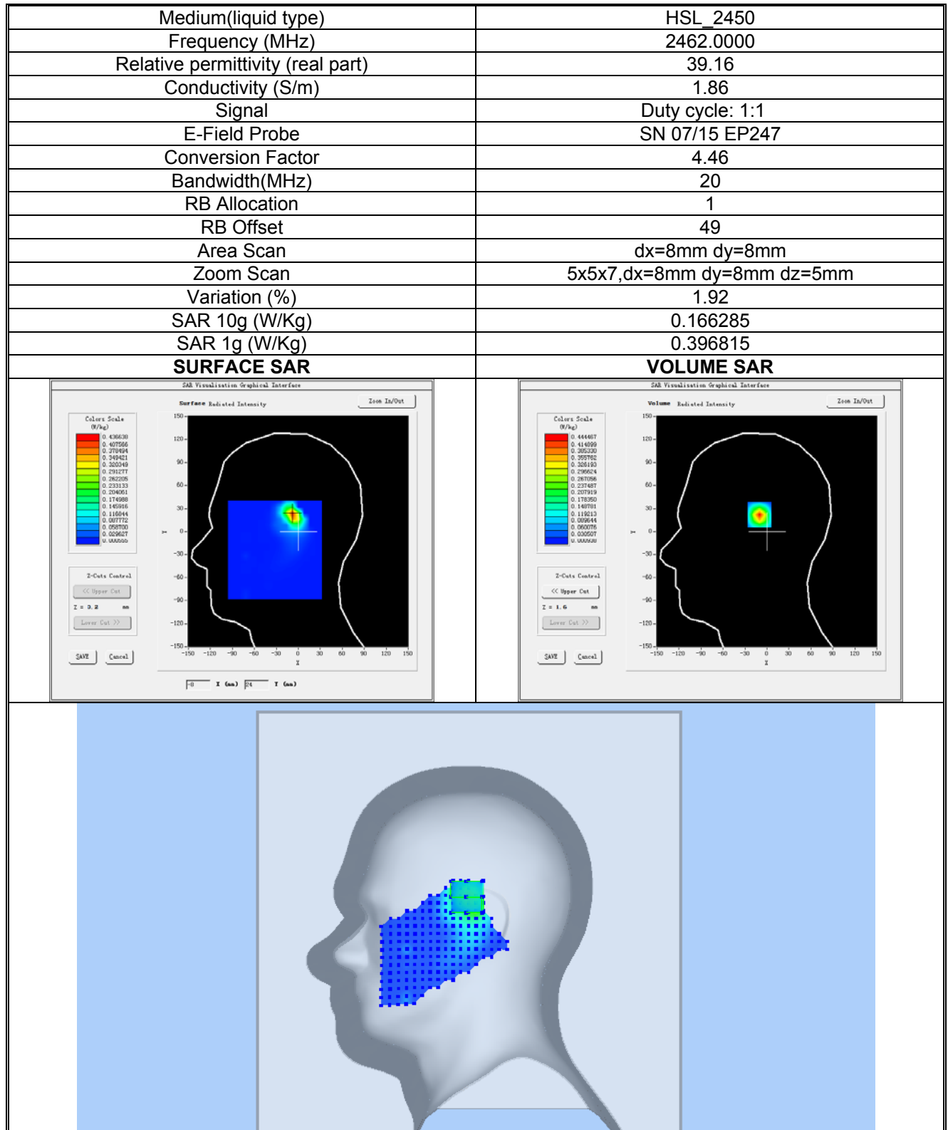
Plot 19:802.11b, High channel (Right Head Tilt) Product Description: Mobile Phone Test Date: 2020-01-13
