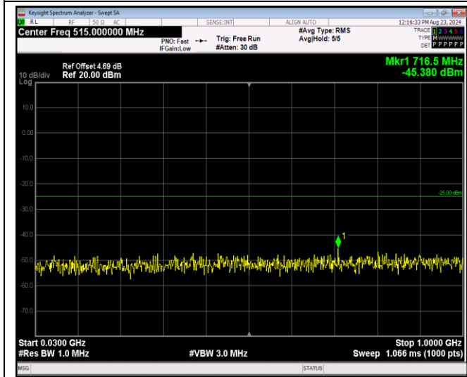
Band41-5MHz-64QAM-40640-1RB#0-Range1:30~100 OMHz
