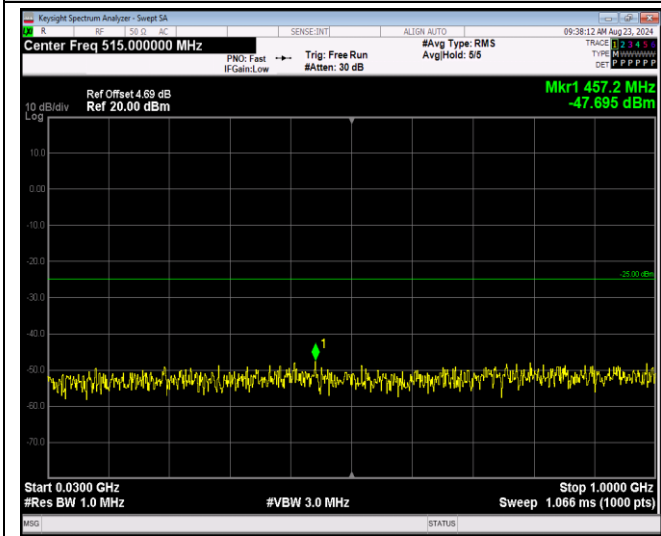
Band7-20MHz-64QAM-20850-1RB#0-Range1:30~100 OMHz
