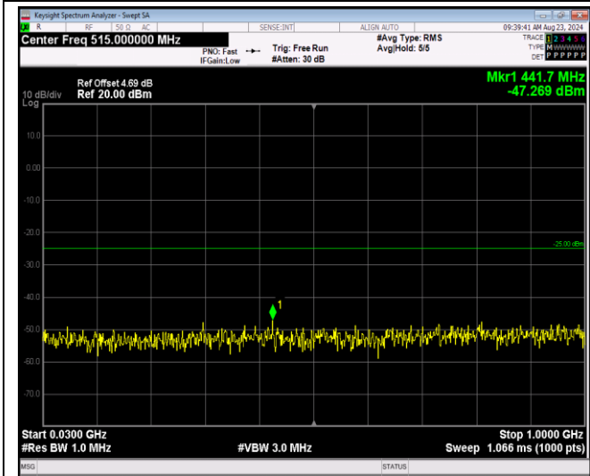
Band7-20MHz-64QAM-20850-1RB#0-Range1:30~100 OMHz
