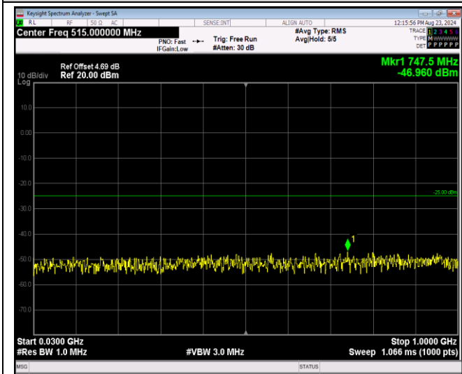
Band41-5MHz-QPSK-41215-1RB#0-Range1:30~1000 MHz
