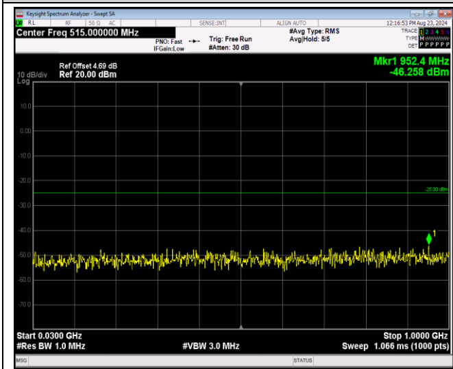
Band41-5MHz-QPSK-41215-1RB#0-Range1:30~1000 MHz
