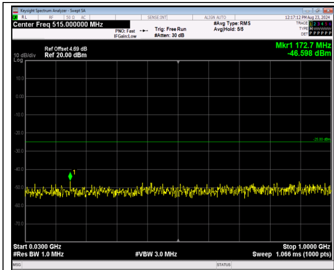
Band41-5MHz-64QAM-40065-1RB#0-Range1:30~100 OMHz
