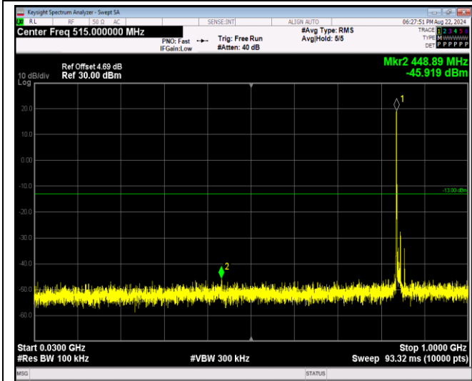
Band7-5MHz-QPSK-20775-1RB#0-Range1:30~1000 MHz
