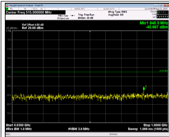
Band41-5MHz-QPSK-40640-1RB#0-Range1:30~1000 MHz
