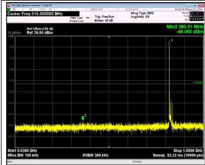
Band5-10MHz-16QAM-20525-1RB#0-Range1:30~100 OMHz
