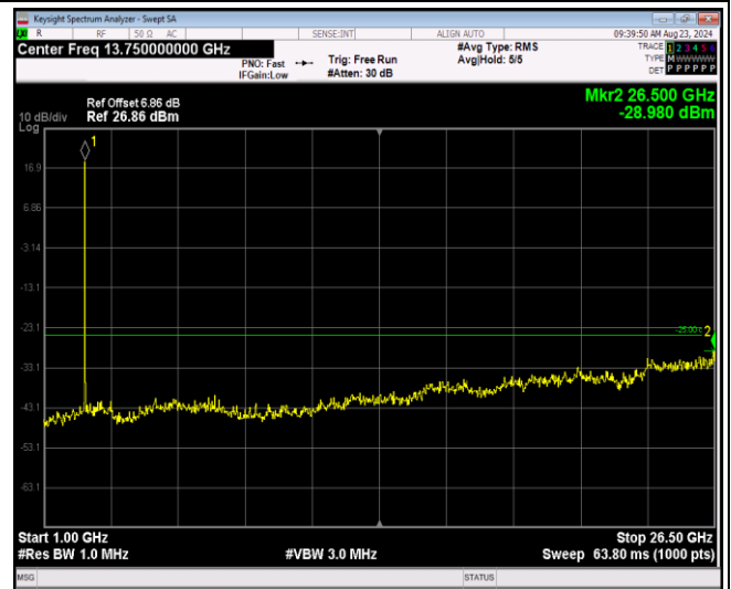
Band7-20MHz-64QAM-20850-1RB#0-Range2:1000~ 26500MHz
