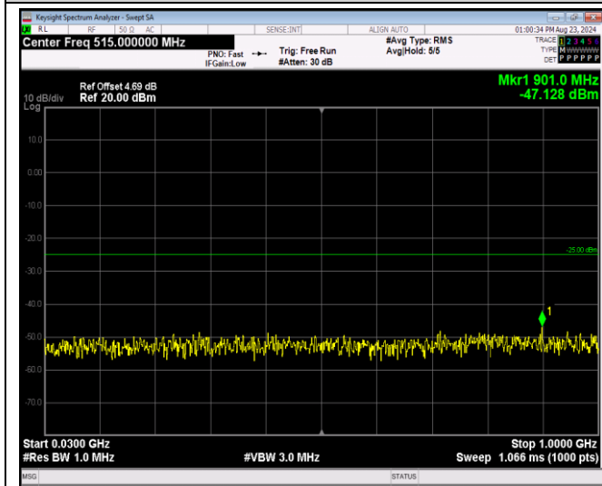
Band41-20MHz-16QAM-40140-1RB#0-Range1:30~10 00MHz
