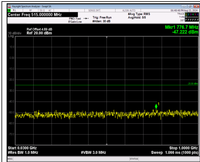
Band7-20MHz-QPSK-20850-1RB#0-Range1:30~1000 MHz
