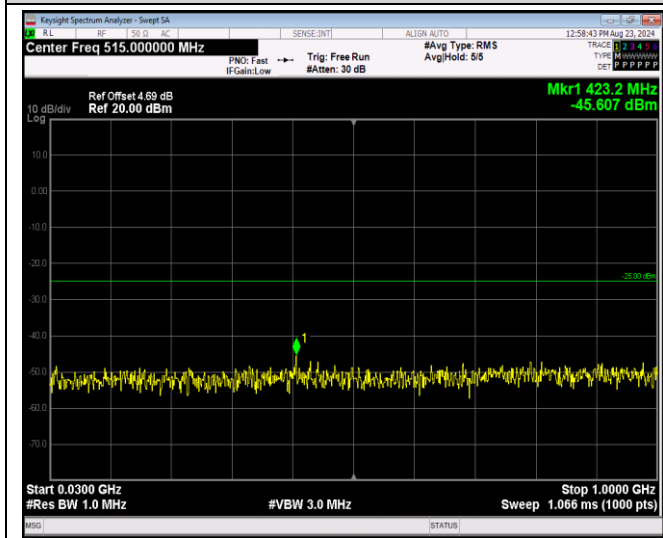
Band41-20MHz-16QAM-40140-1RB#0-Range1:30~10 00MHz
