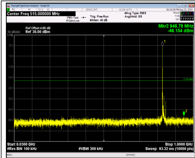
Band5-10MHz-64QAM-20600-1RB#0-Range1:30~100 OMHz
