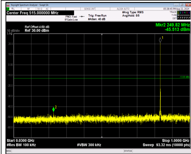
Band5-1.4MHz-64QAM-20643-1RB#0-Range1:30~1000MHz
