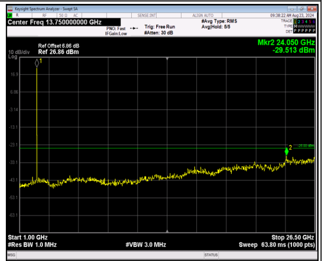
Band7-20MHz-64QAM-20850-1RB#0-Range2:1000~ 26500MHz
