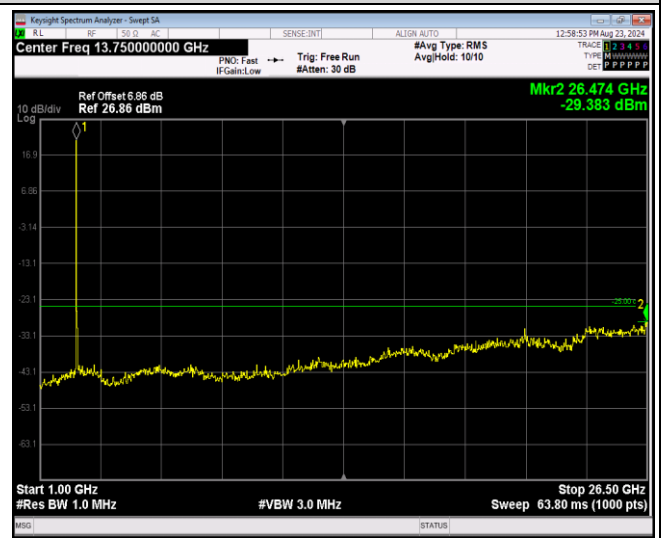
Band41-20MHz-16QAM-40140-1RB#0-Range2:1000 ~26500MHz
