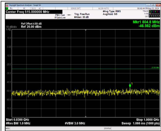
Band7-5MHz-16QAM-21100-1RB#0-Range1:30~1000 MHz
