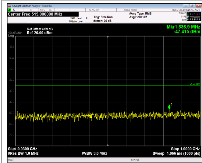
Band7-20MHz-QPSK-21100-1RB#0-Range1:30~1000 MHz
