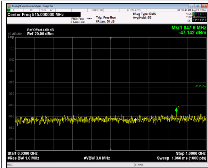
Band7-20MHz-16QAM-21350-1RB#0-Range1:30~100 OMHz
