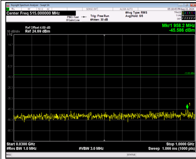
Band4-20MHz-QPSK-20300-1RB#0-Range1:30~1000 MHz
