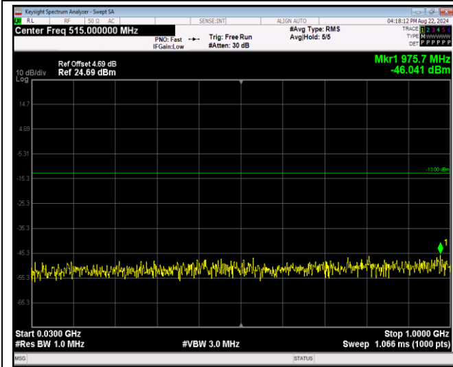
Band4-1.4MHz-QPSK-20175-1RB#0-Range1:30~100 OMHz
