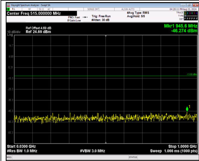
Band4-1.4MHz-64QAM-19957-1RB#0-Range1:30~1000MHz
