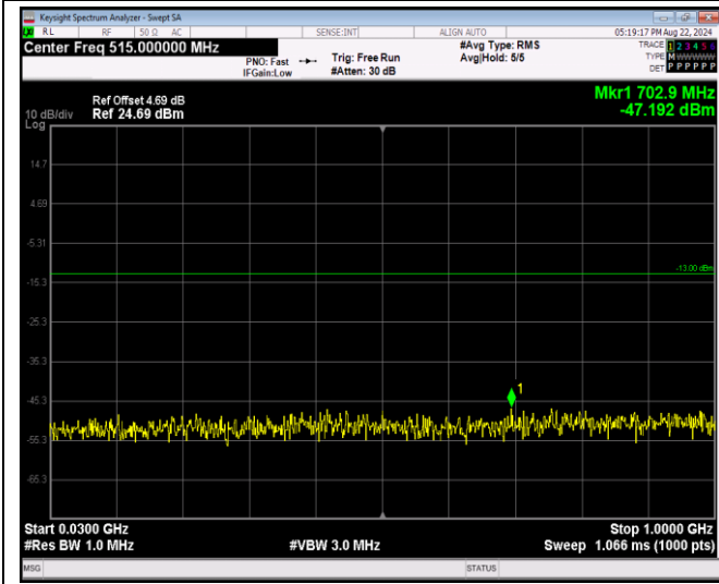
Band4-20MHz-64QAM-20175-1RB#0-Range1:30~100 OMHz
