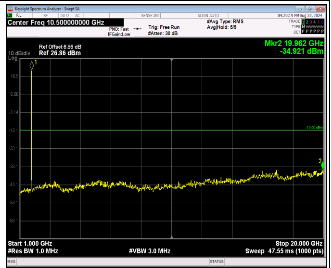
Band4-1.4MHz-64QAM-19957-1RB#0-Range2:1000~20000MHz
