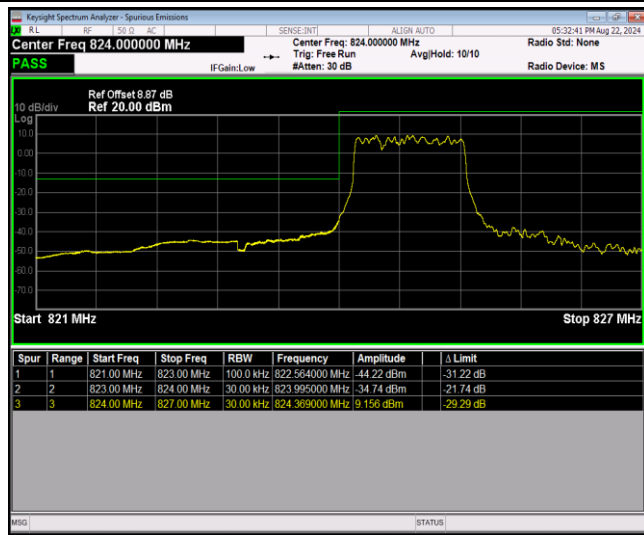
Band5-1.4MHz-QPSK-20643-1RB#5
