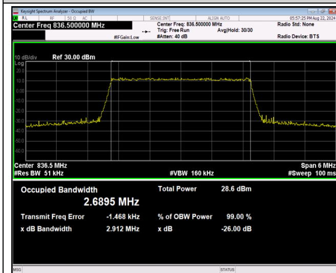
Band5-5MHz-QPSK-20425-25RB#0
