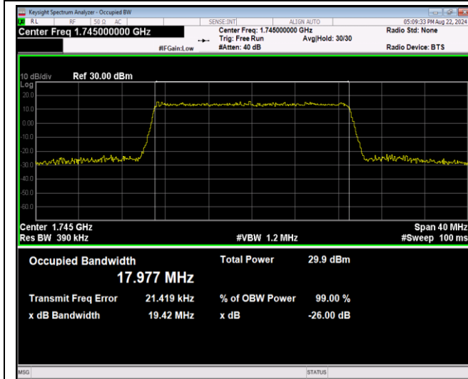
Band4-20MHz-64QAM-20175-100RB#0
