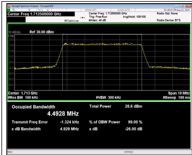
Band4-5MHz-64QAM-20375-25RB#0
