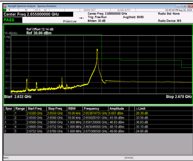
Band41-20MHz-64QAM-41140-1RB#99
