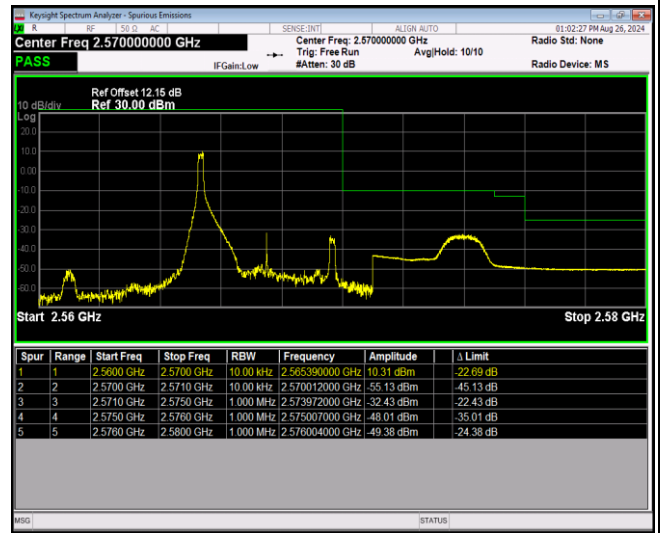
Band7-5MHz-64QAM-21425-25RB#0
