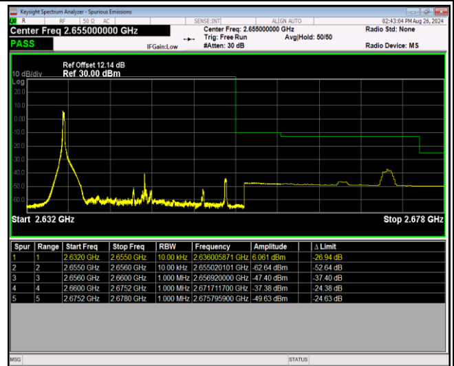
Band41-20MHz-16QAM-41140-100RB#0
