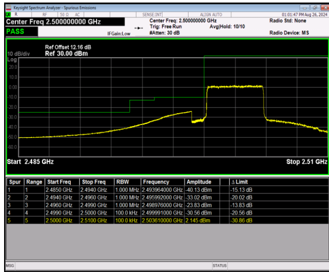
Band7-5MHz-64QAM-21425-1RB#24
