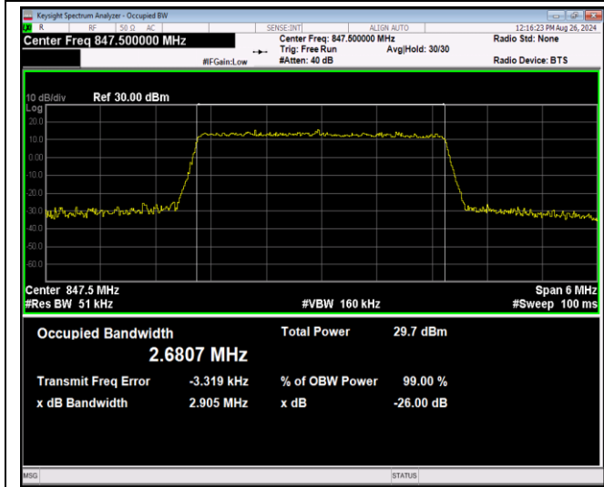
Band5-3MHz-64QAM-20525-15RB#0
