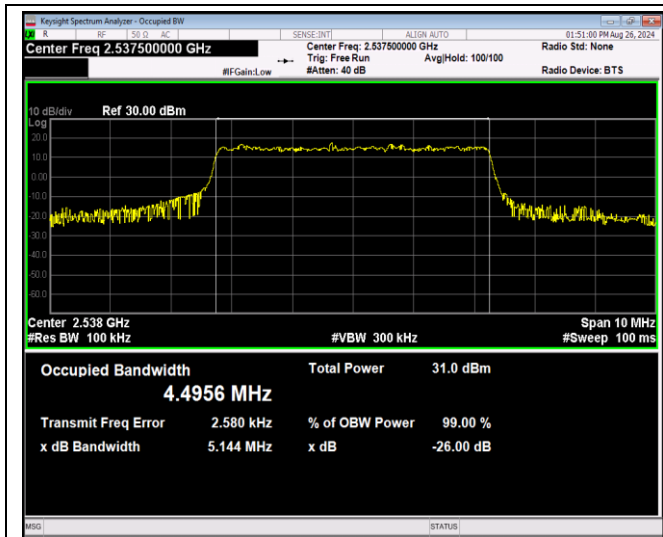
Band41-5MHz-QPSK-41215-25RB#0
