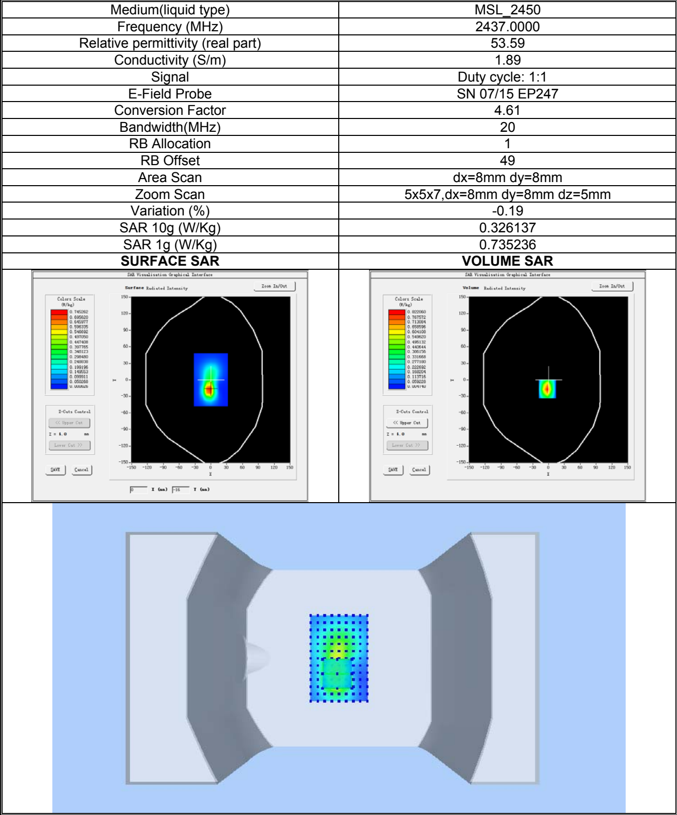
Plot 21: 802.11b, Mid channel (Hotspot, Top Edge) Product Description: Mobile Phone Test Date: 2019-10-15
