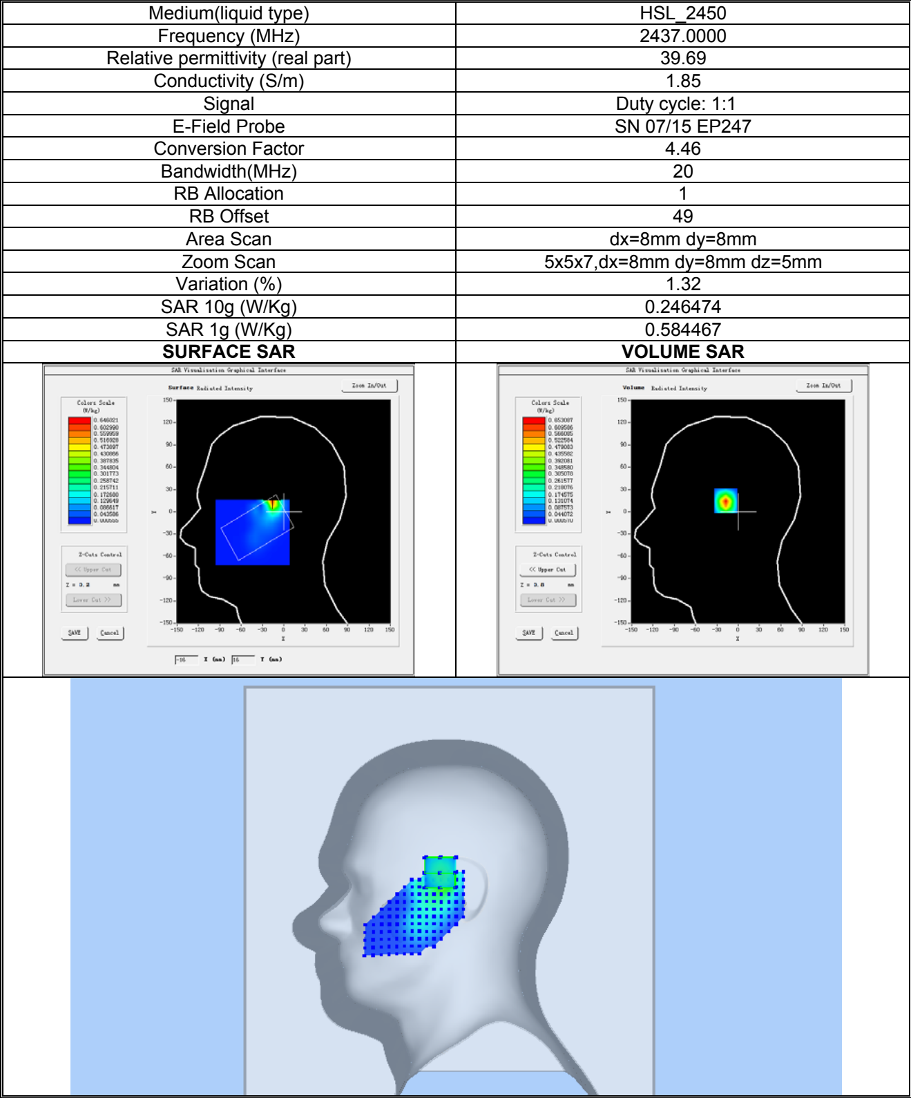
Plot 19:802.11b, Mid channel (Right Head Cheek) Product Description:Mobile Phone Test Date: 2019-10-15
