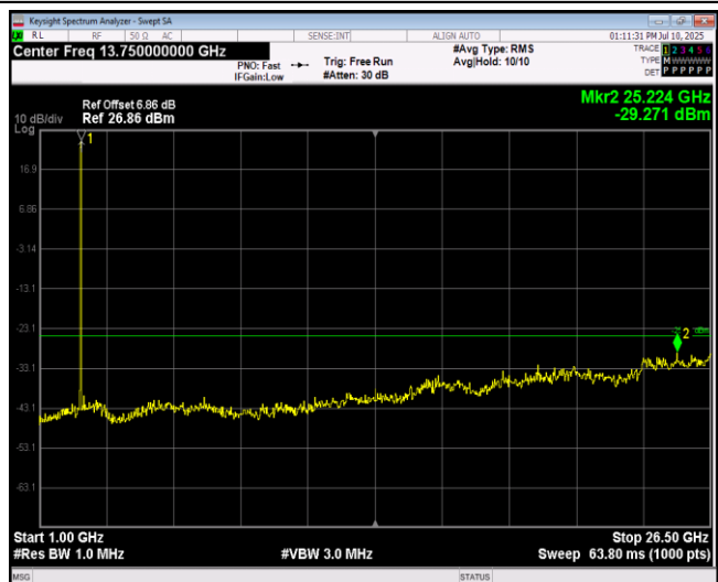
Band38-5MHz-16QAM-38000-1RB#0-Range2:1000~ 26500MHz
