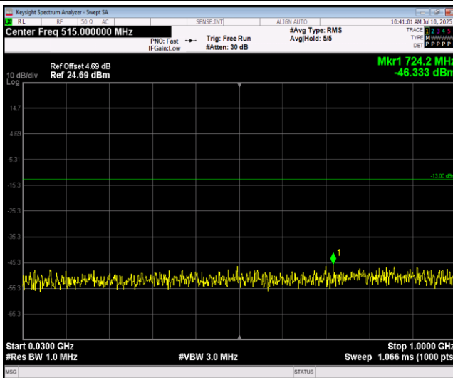
Band25-20MHz-QPSK-26590-1RB#0-Range1:30~1000MHz
