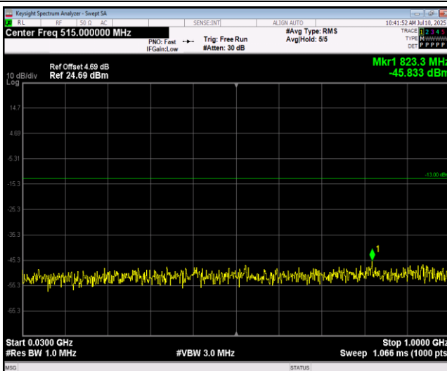
Band25-20MHz-16QAM-26140-1RB#0-Range1:30~1000MHz
