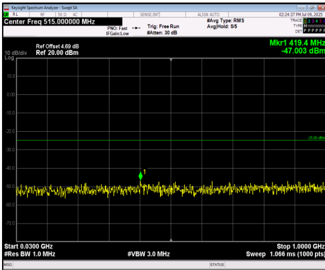
Band7-5MHz-64QAM-21100-1RB#0-Range1:30~100 0MHz
