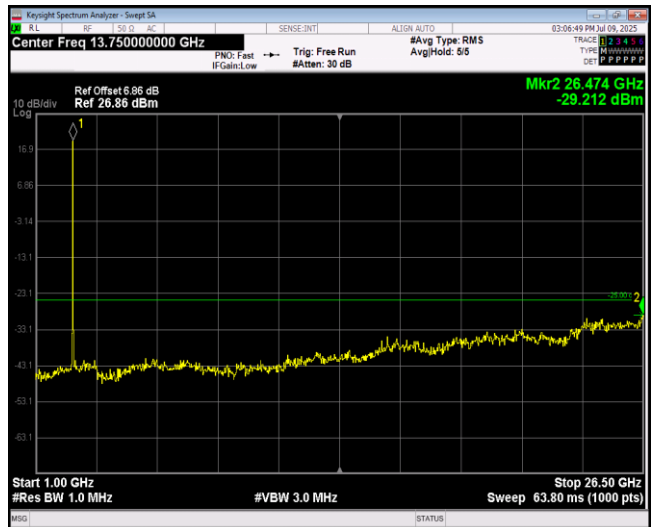
Band7-20MHz-16QAM-20850-1RB#0-Range2:1000~ 26500MHz
