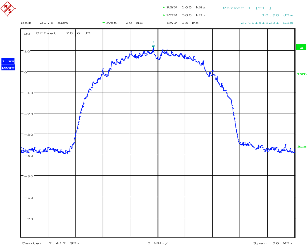
Reference plot 2412 MHz 802.11b
