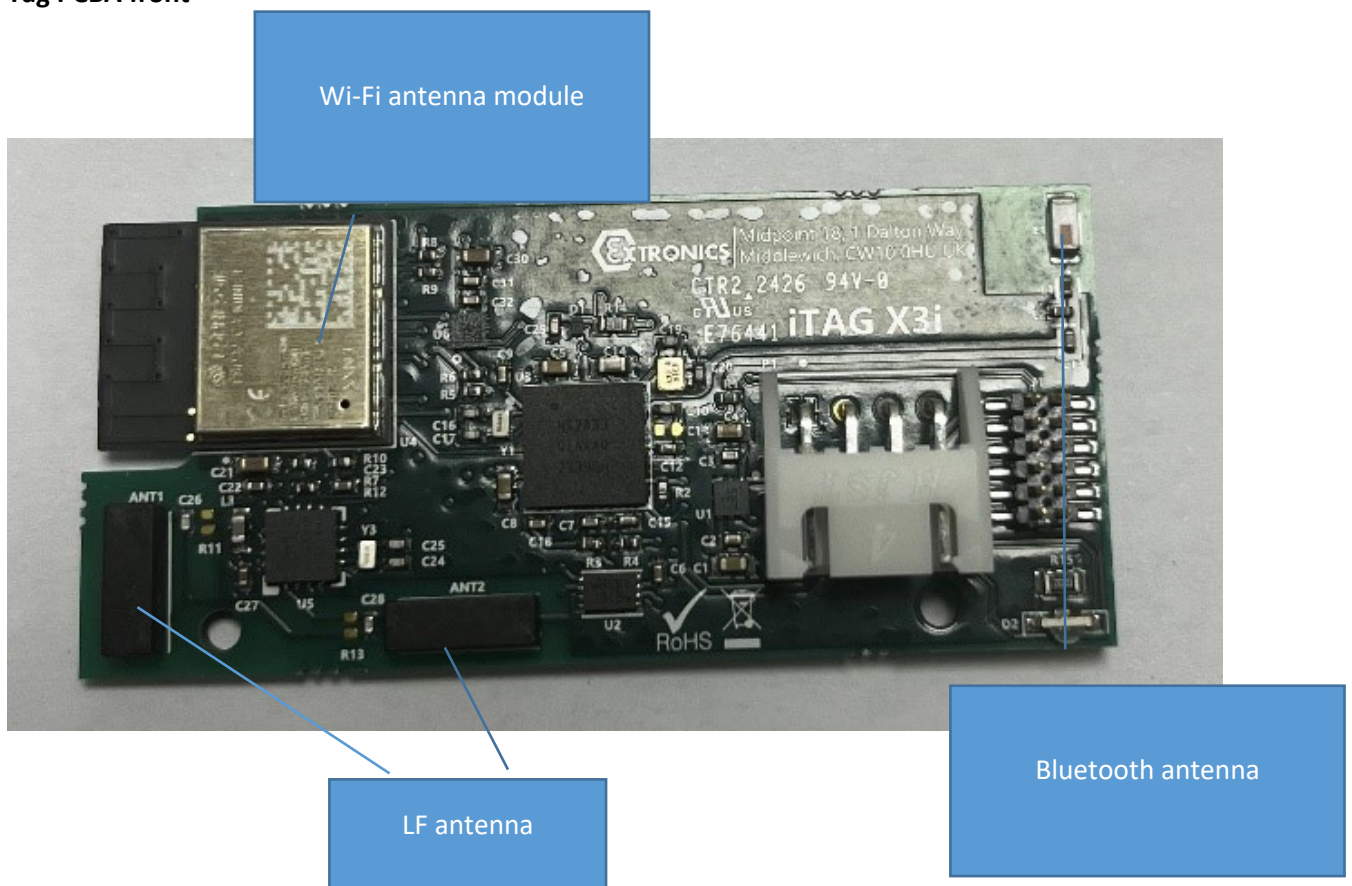
Tag PCBA front
