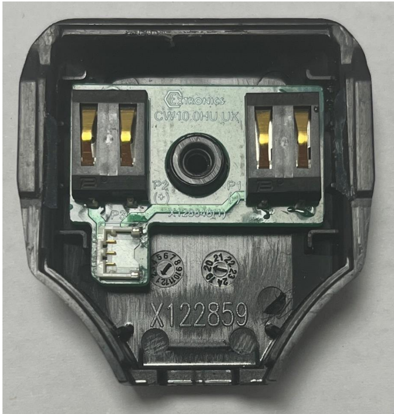
Charger PCBA in charger cover
