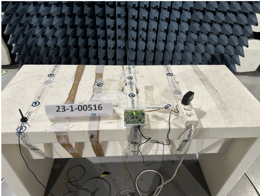
Photograph 7: EUT test setup in the semi anechoic chamber, close up view_EUT elevation 0°
