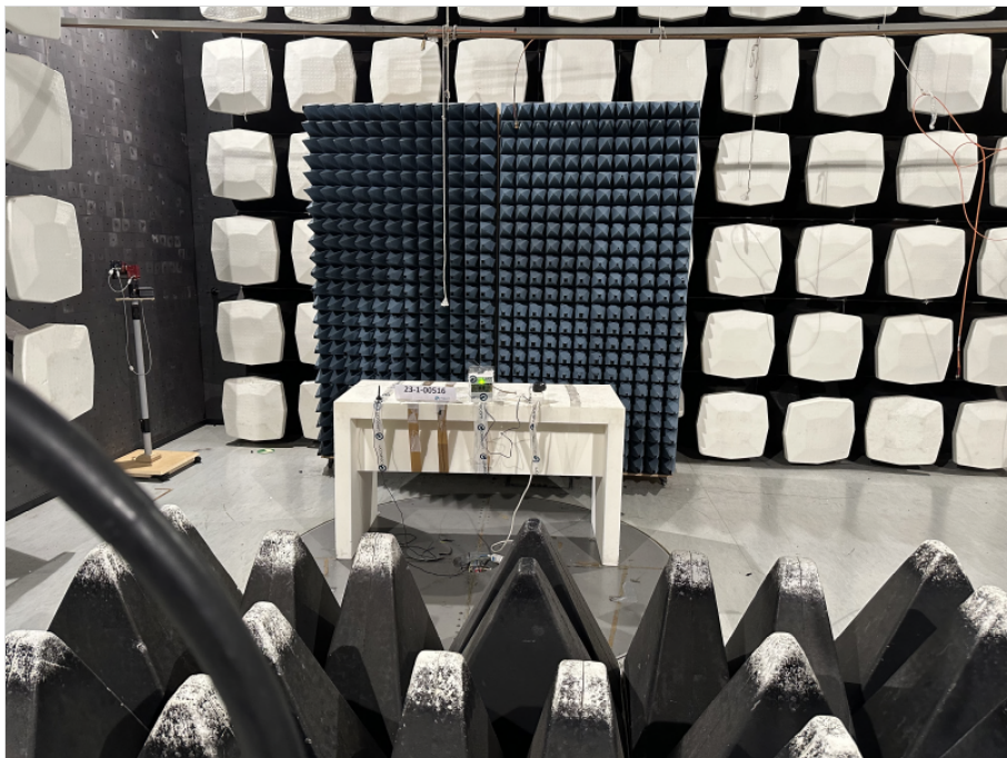
Photograph 10: EUT test setup in the semi anechoic chamber, overview_EUT elevation 90°
