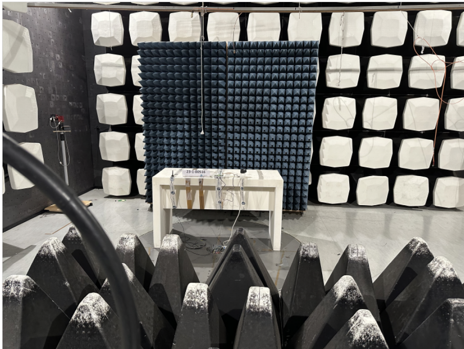
Photograph 8: EUT test setup in the semi anechoic chamber, overview_EUT elevation 0°
