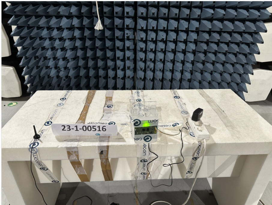
Photograph 9: EUT test setup in the semi anechoic chamber, close up view_EUT elevation 90°
