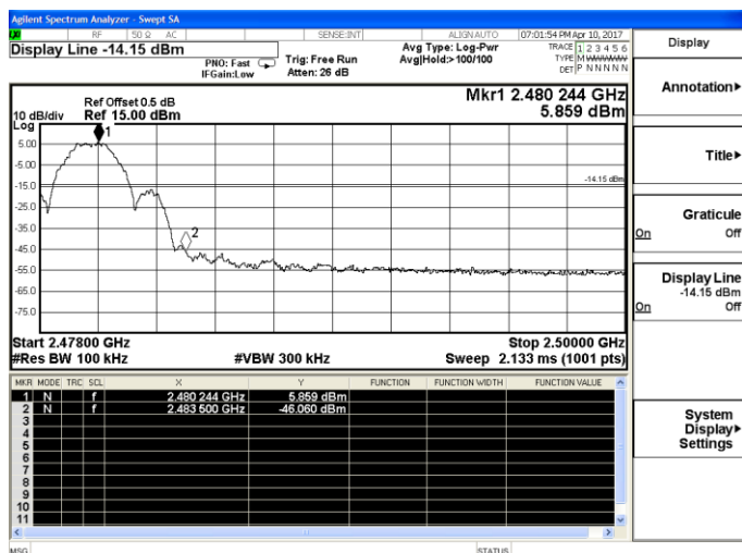
Channel 15 / 2480 MHz
