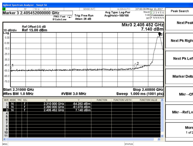
Channel 0 / 2405 MHz – Peak
