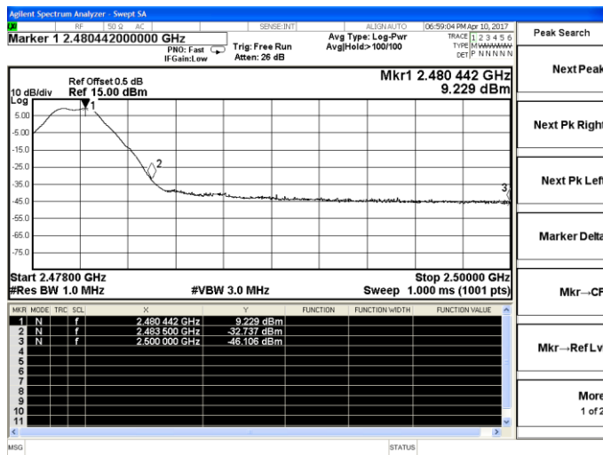
Channel 15 / 2480 MHz – Peak
