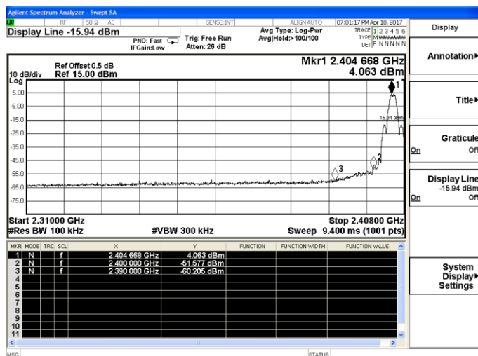
Channel 0 / 2405 MHz
