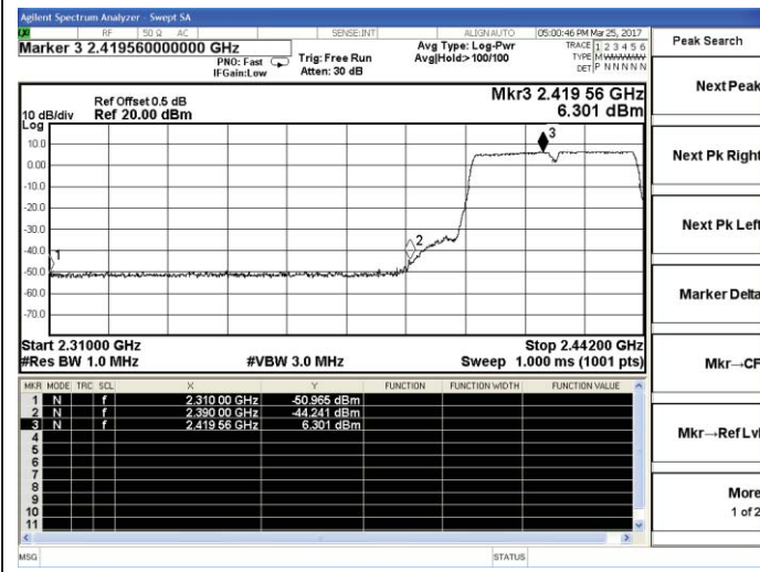
802.11n-HT40-Low channel(Peak)
