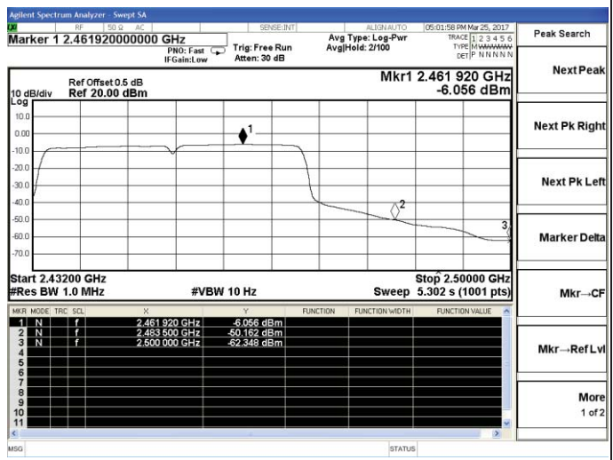
802.11n-HT40-High channel(Average)
