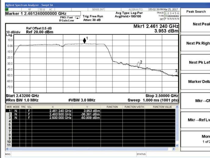
802.11n-HT40-High channel(Peak)
