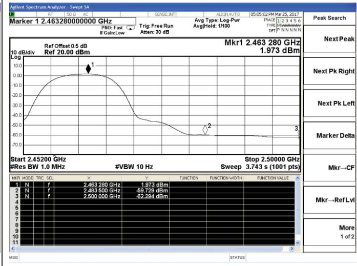
802.11b-High channel(Average)
