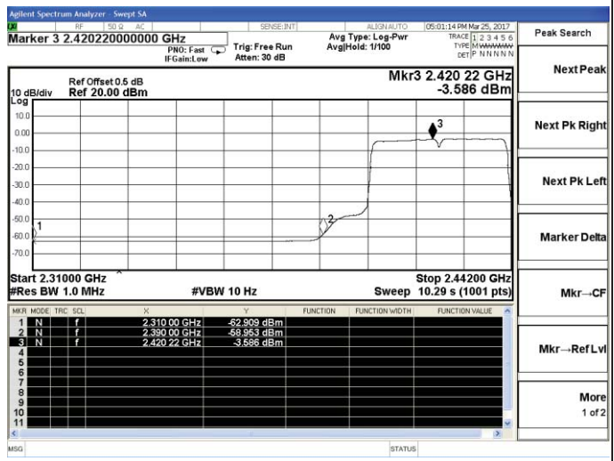
802.11n-HT40-Low channel(Average)
