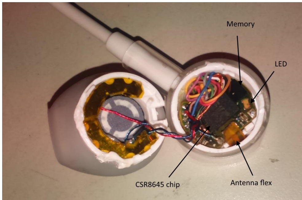
Main PCB from the front with mechanics.
