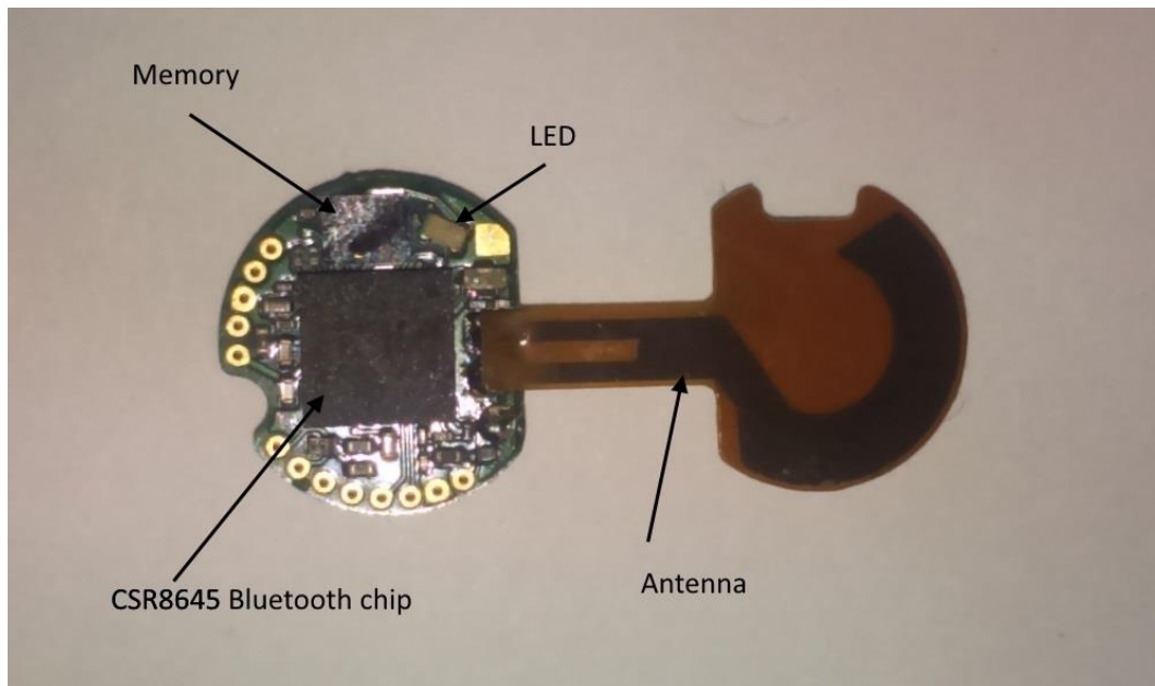
Main PCB from the front (clearer picture)
