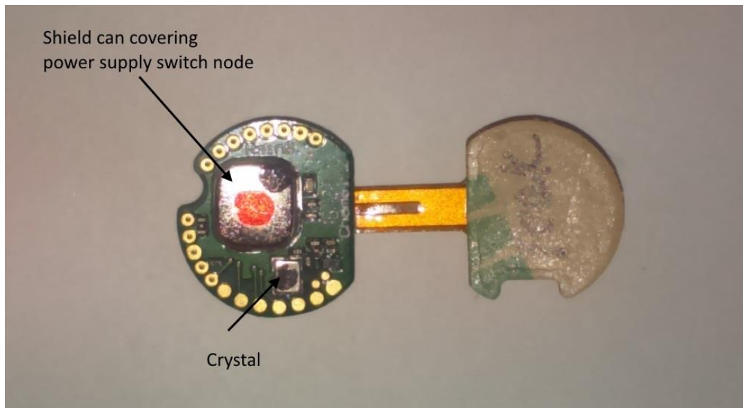
Main PCB from the back (clearer picture).
