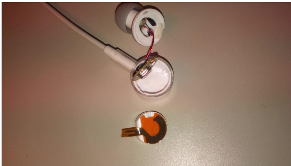
Better view of the antenna with plastic carrier.
