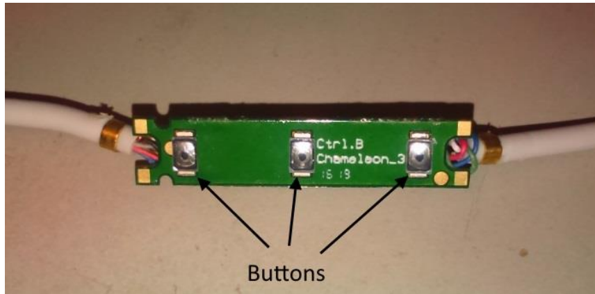
Control box PCB from the back.
