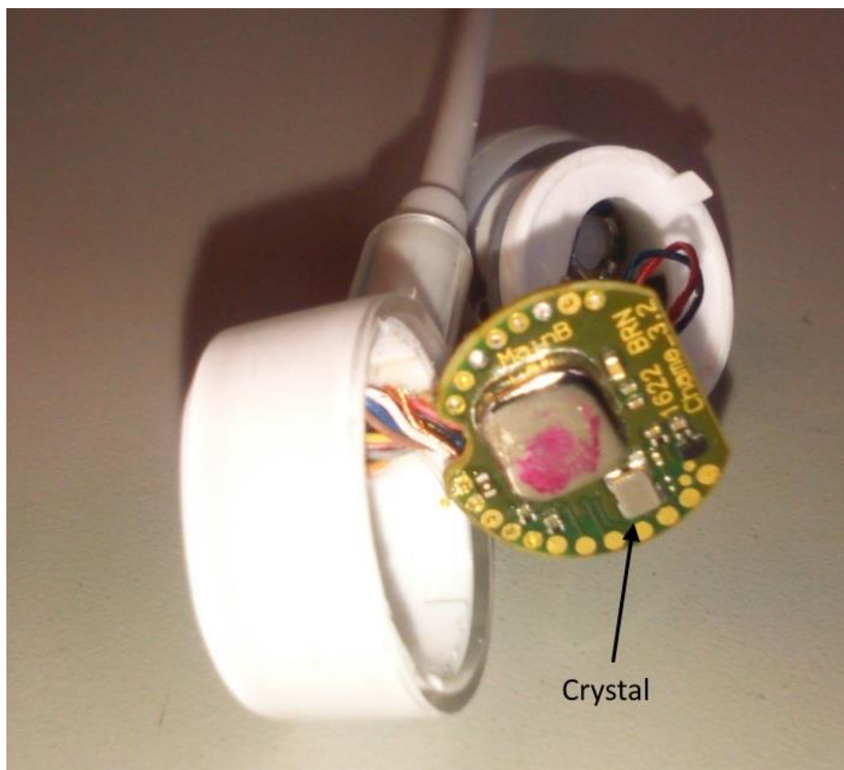
Main PCB from the back with mechanics.
