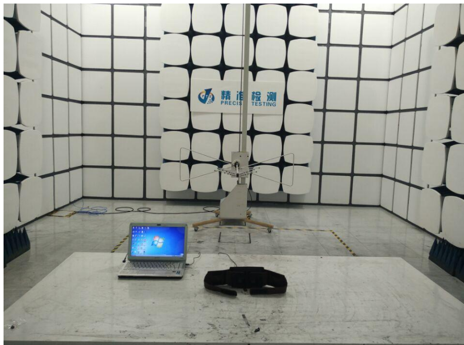
Test Setup DTS From 30MHz-1000MHz
