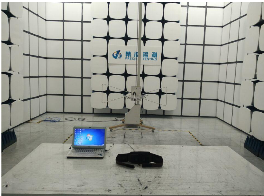
Test SETUP DSS From 30MHz-1000MHz
