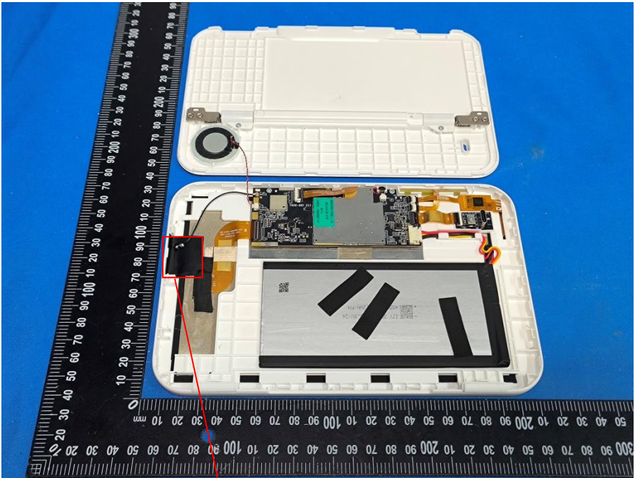
WIFI/Bluetooth Ant
