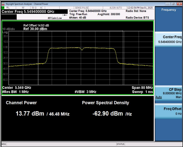
11N40SISO-Ant1-5550-PASS
