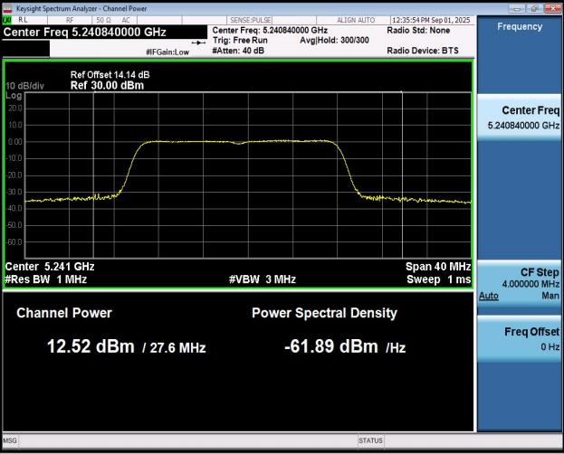
11AC20SISO-Ant1-5240-PASS
