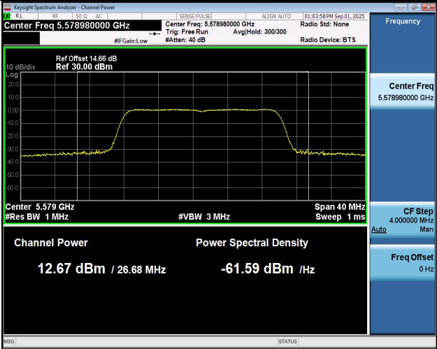
11AC20SISO-Ant1-5580-PASS
