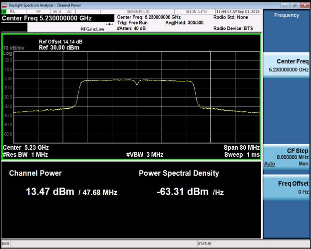
11N40SISO-Ant1-5230-PASS
