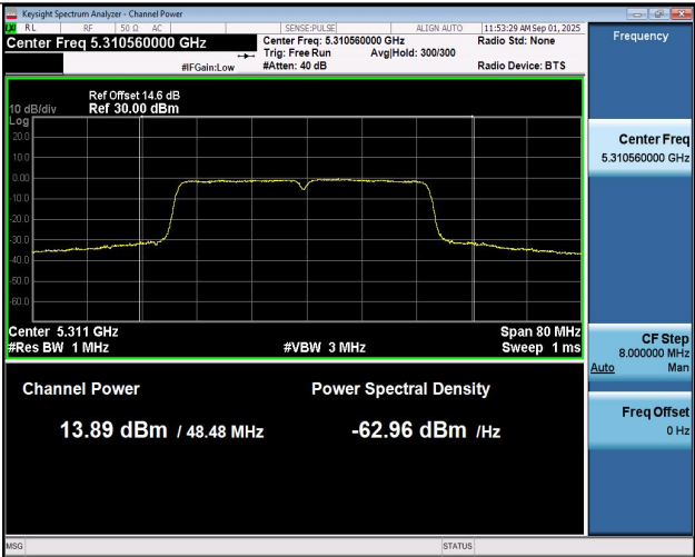
11N40SISO-Ant1-5310-PASS
