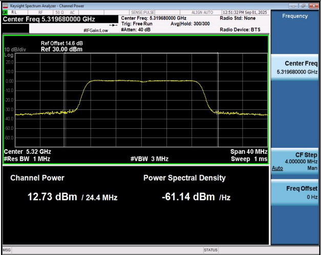
11AC20SISO-Ant1-5320-PASS
