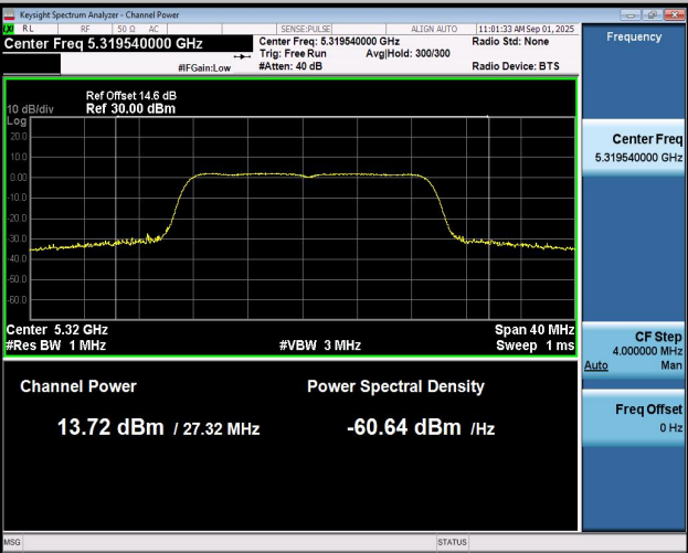
11N20SISO-Ant1-5320-PASS
