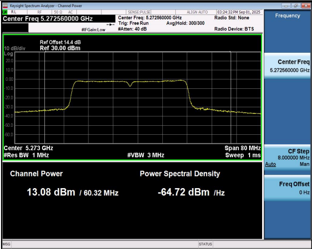
11AC40SISO-Ant1-5270-PASS
