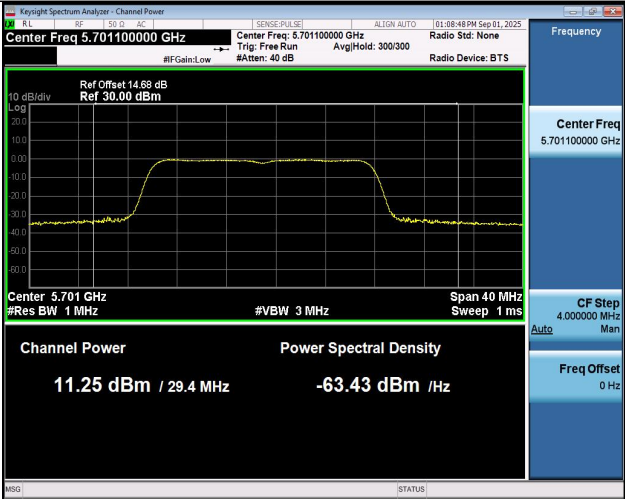
11AC20SISO-Ant1-5700-PASS
