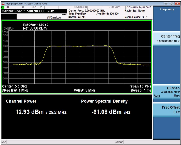
11AC20SISO-Ant1-5500-PASS
