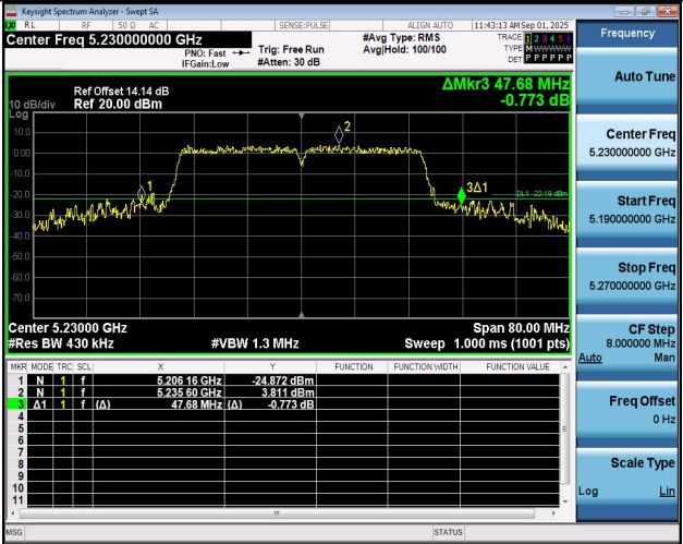
11N40SISO-Ant1-5230
