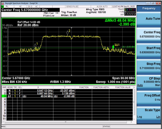
11N40SISO-Ant1-5670
