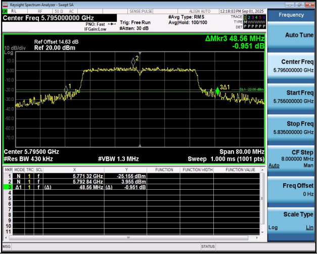
11N40SISO-Ant1-5795
