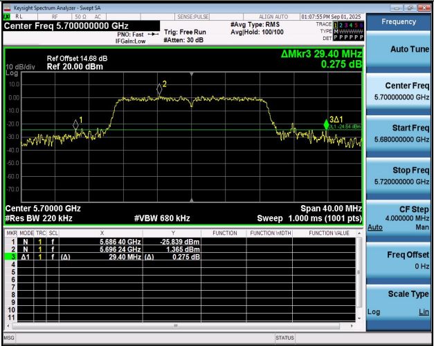
11AC20SISO-Ant1-5700
