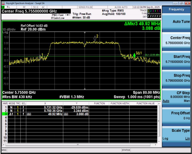
11N40SISO-Ant1-5755
