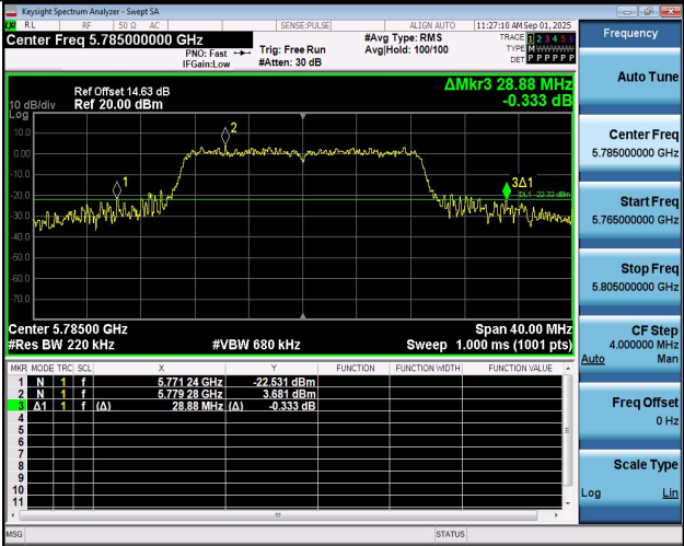
11N20SISO-Ant1-5785
