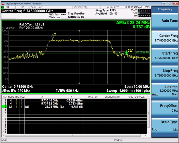
11N20SISO-Ant1-5745
