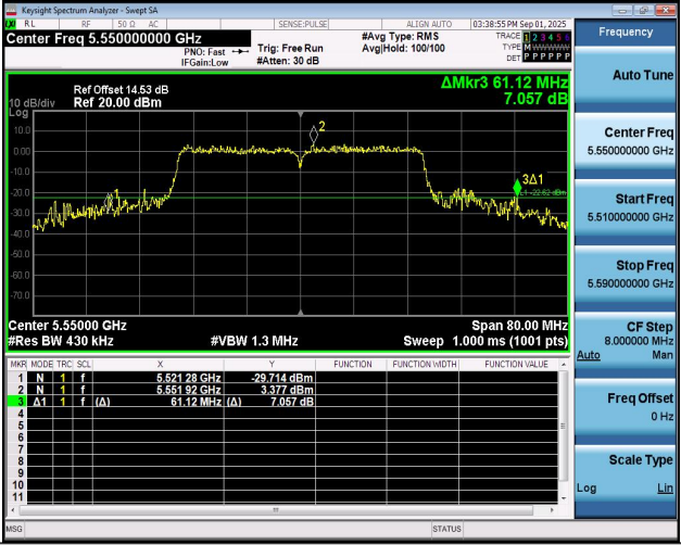
11AC40SISO-Ant1-5550
