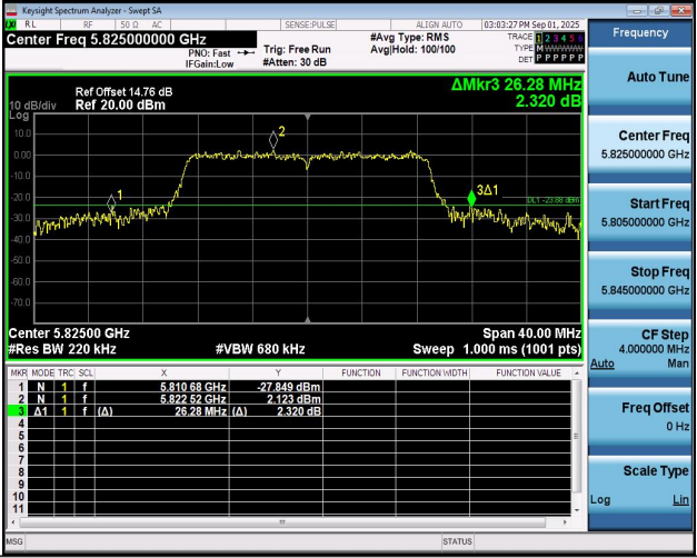
11AC20SISO-Ant1-5825
