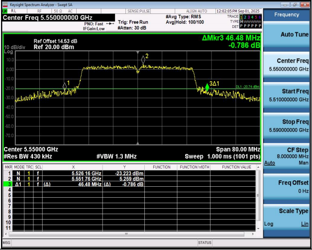
11N40SISO-Ant1-5550
