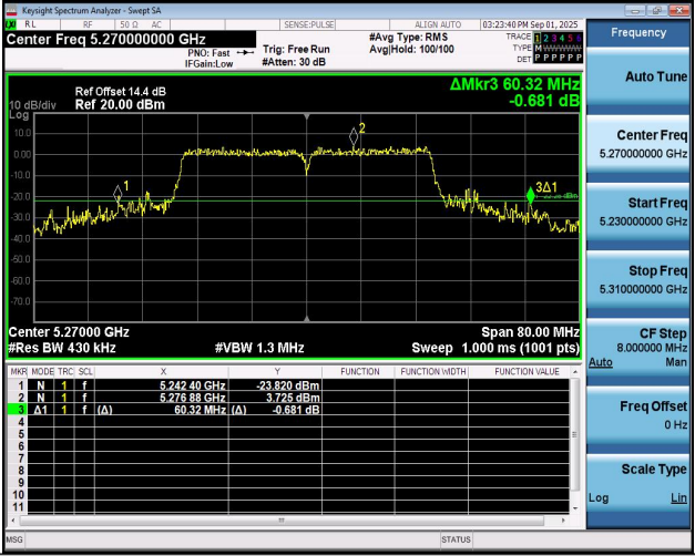
11AC40SISO-Ant1-5270
