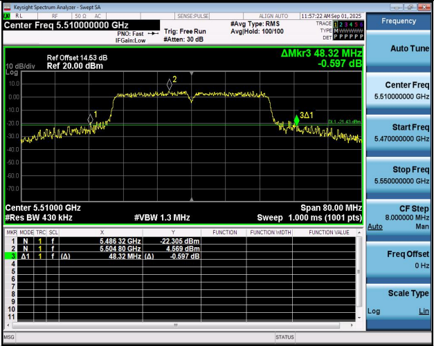
11N40SISO-Ant1-5510
