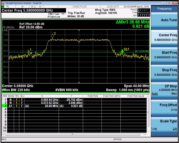
11AC20SISO-Ant1-5580
