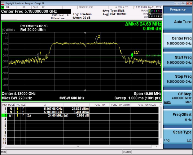
11AC20SISO-Ant1-5180
