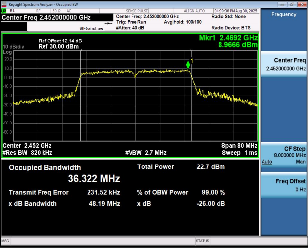
11N40SISO-Ant1-2452
