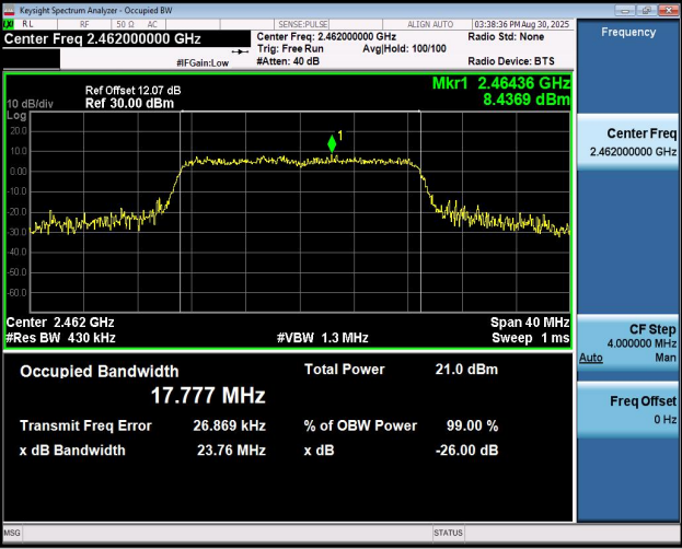
11N20SISO-Ant1-2462
