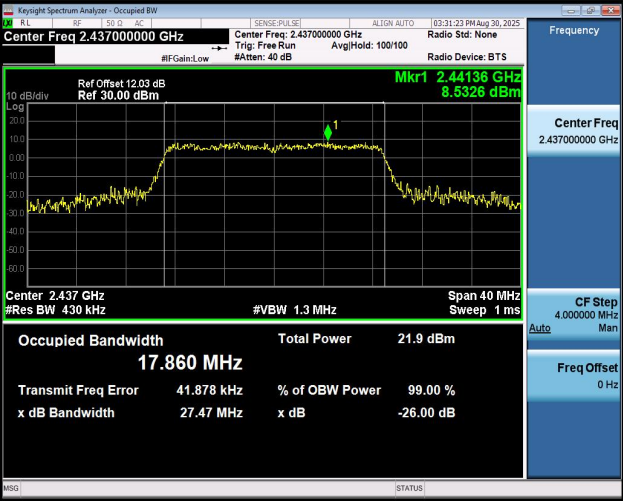
11N20SISO-Ant1-2437
