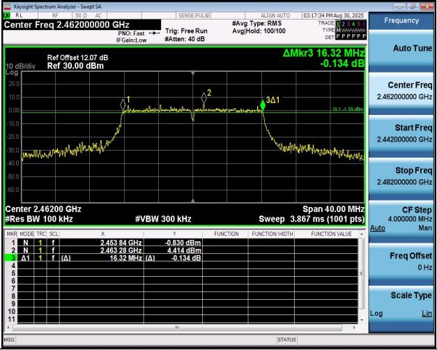
11G-Ant1-2462-PASS
