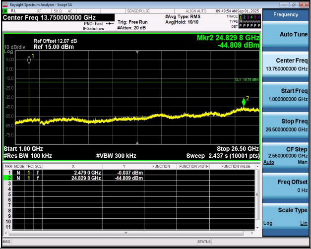
LE_1M-Ant1-2480-1000~26500-PASS
