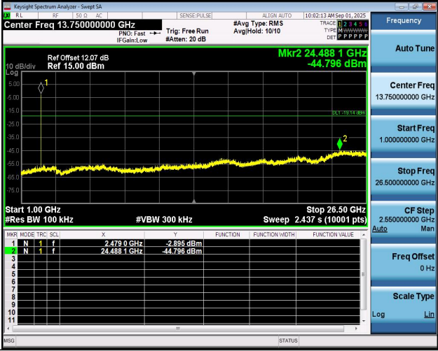
LE_2M-Ant1-2480-1000~26500-PASS
