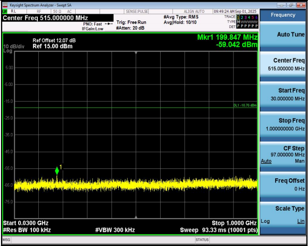
LE_1M-Ant1-2480-30~1000-PASS
