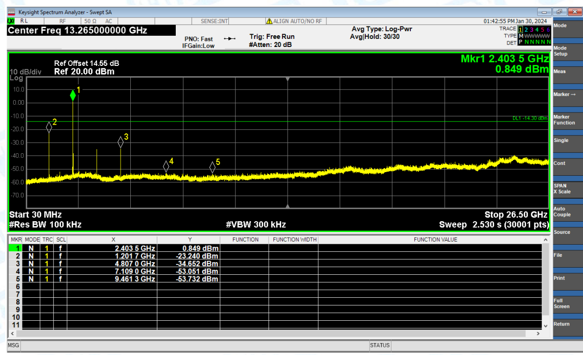
Tx. Spurious NVNT 2404MHz Emission
