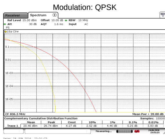
LTE Band 5 Middle channel
