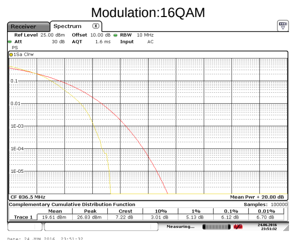
LTE Band 5 Middle channel
