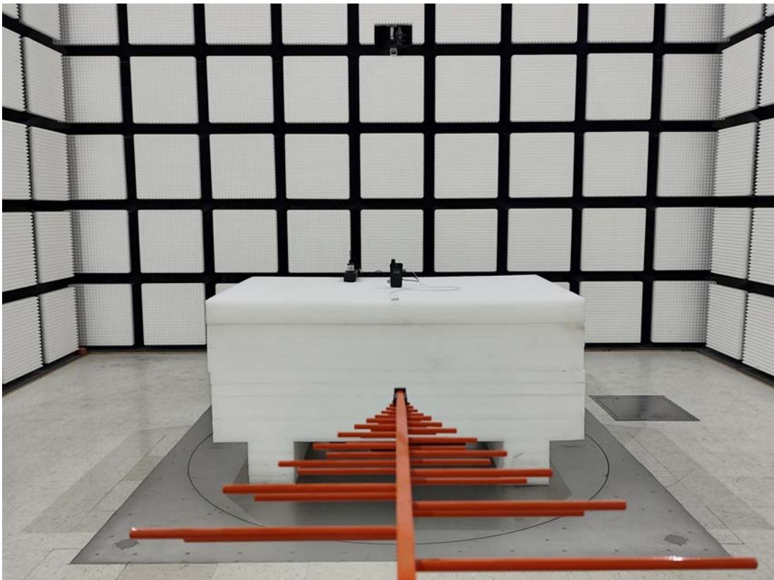
Radiated Emission Below 1GHz View Without Charging Base:
