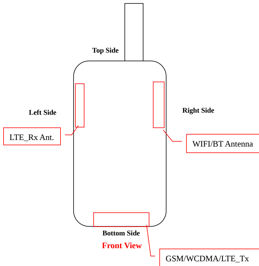
Block Diagram for EUT Antenna Position
