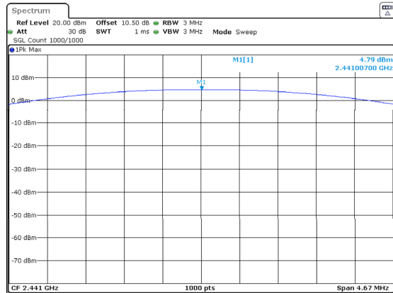
DH1_Middle 4.79dBm
