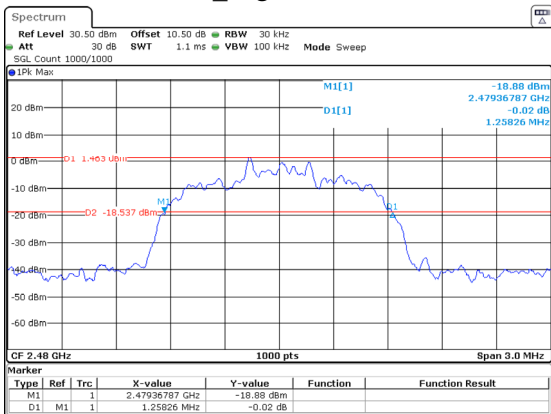
2DH1_High 1.258MHz
