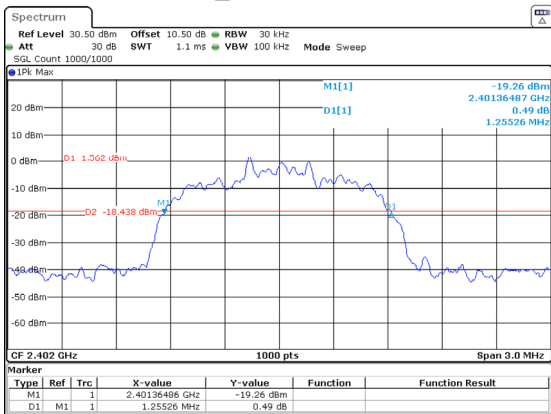
2DH1_Low 1.255MHz
