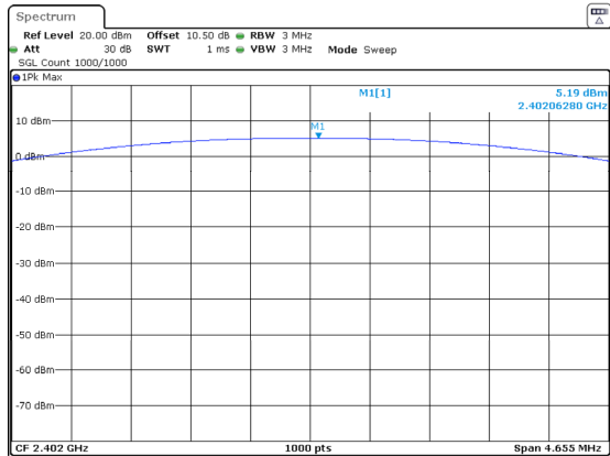
DH1_Low 5.19dBm
