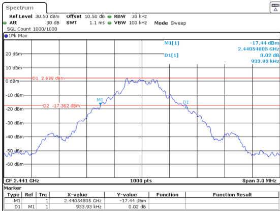
DH1_Middle 0.934MHz
