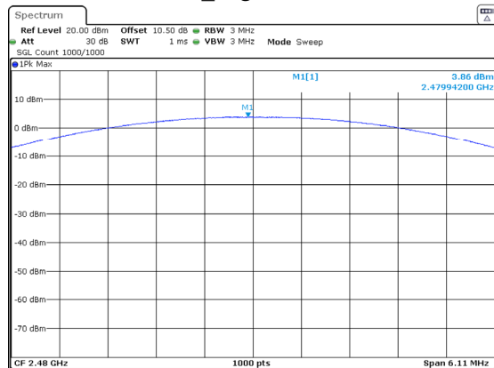
2DH1_High 3.86dBm
