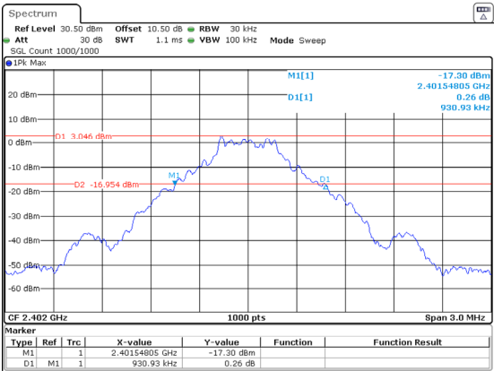
DH1_Low 0.931MHz
