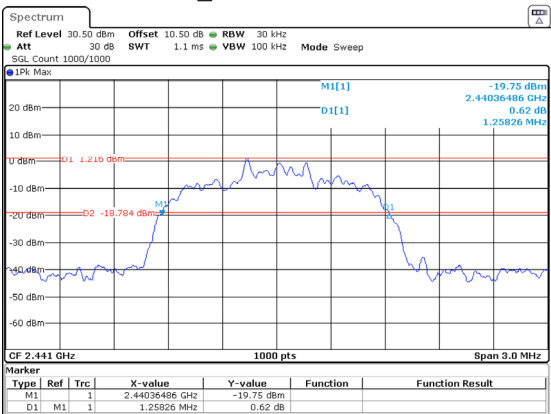
2DH1_Middle 1.258MHz
