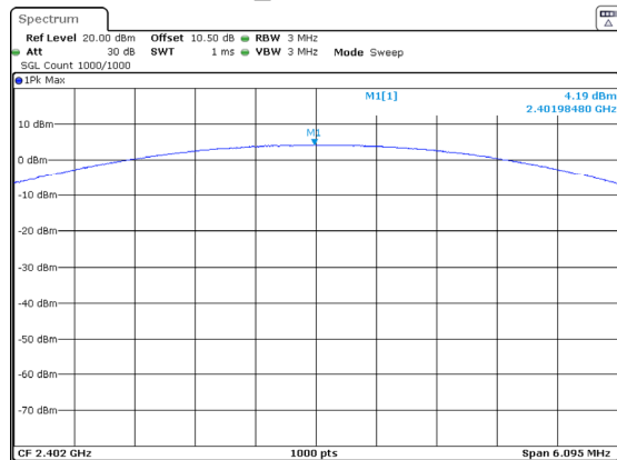
2DH1_Low 4.19dBm
