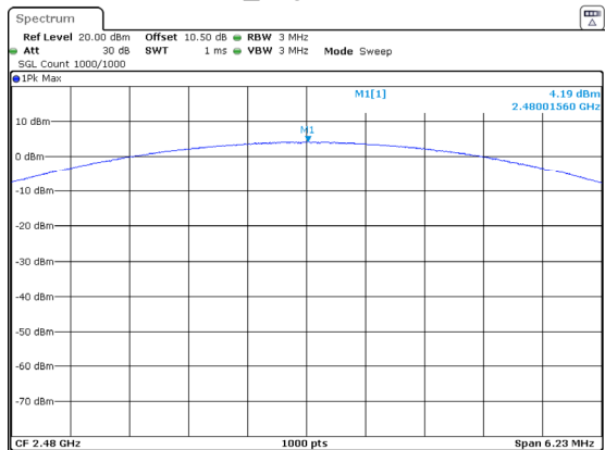
3DH1_High 4.19dBm
