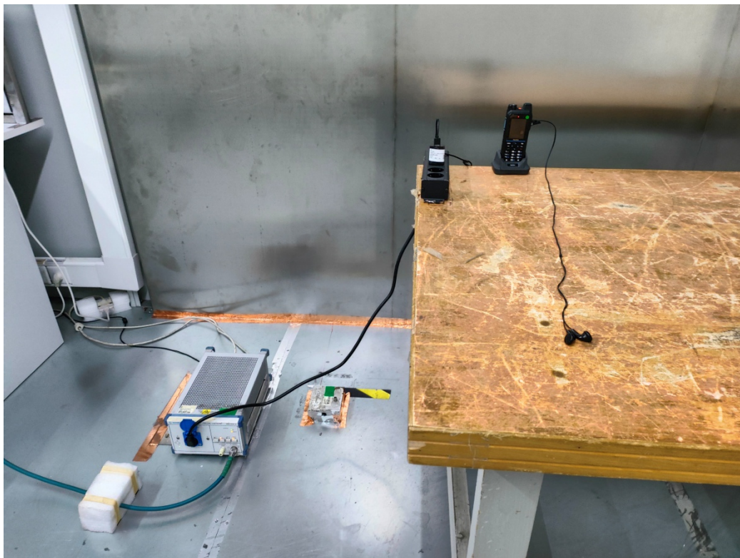
Conducted Emissions - Side View-Charger
