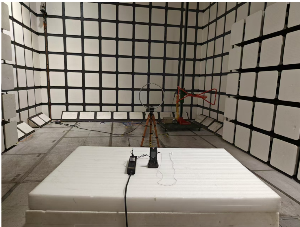
Radiated Emissions View (Below 30MHz)-Charger
