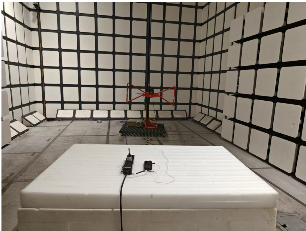
Radiated Emissions View (Below 1 GHz) -Adapter
