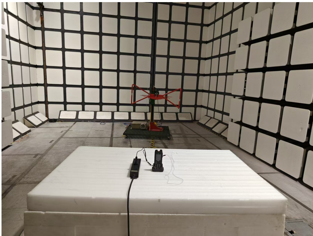
Radiated Emissions View (Below 1 GHz)-Charger
