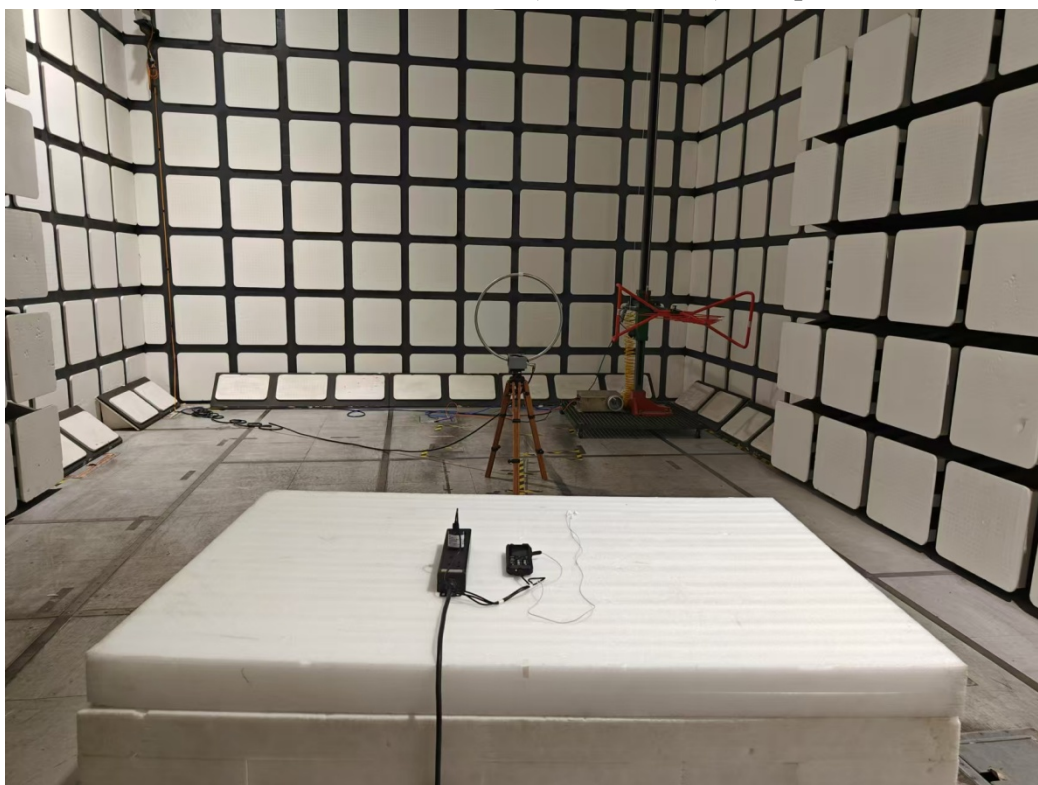
Radiated Emissions View (Below 30MHz) -Adapter
