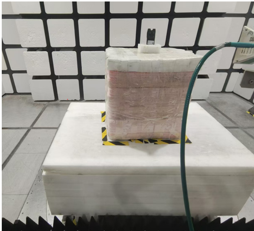
Radiated Emissions View (18-40 GHz)
