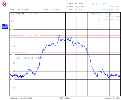
2DH1_High 1.219MHz
