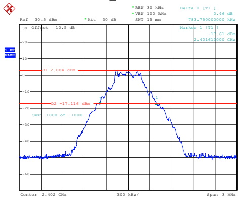
DH1_Low 0.784MHz
