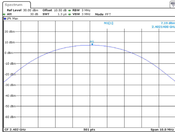
DH1_Low 7.19dBm
