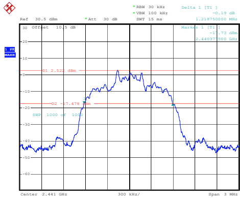
2DH1_Middle 1.219MHz
