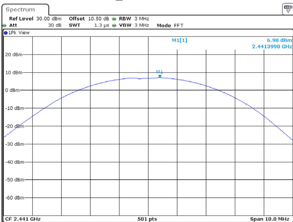
3DH1_Middle 6.98dBm
