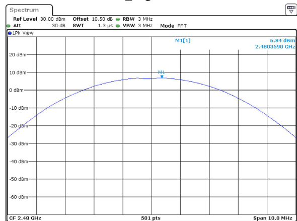
3DH1_High 6.84dBm
