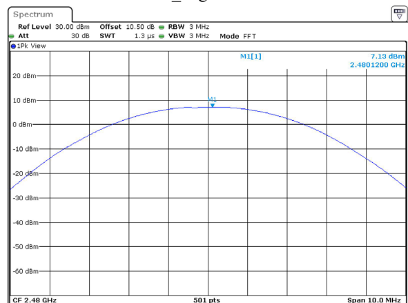
2DH1_High 7.13dBm
