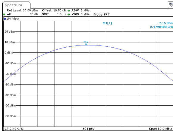
DH1_High 7.15dBm
