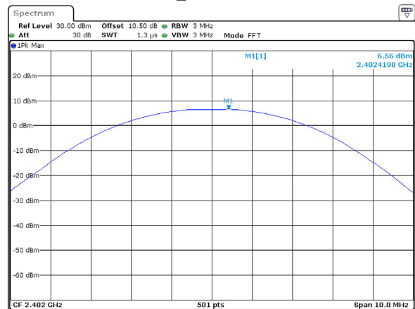
3DH1_Low 6.56dBm
