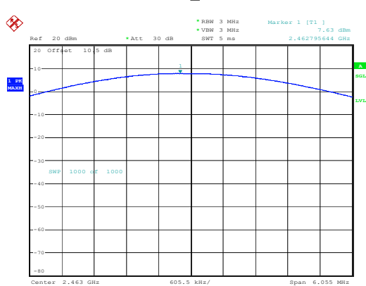
2DH1_Additional
