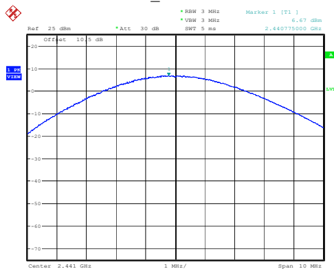
2DH1_Middle 6.67dBm
