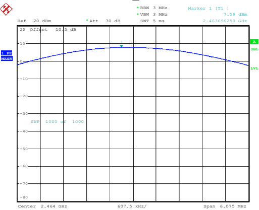
3DH1_Additional
