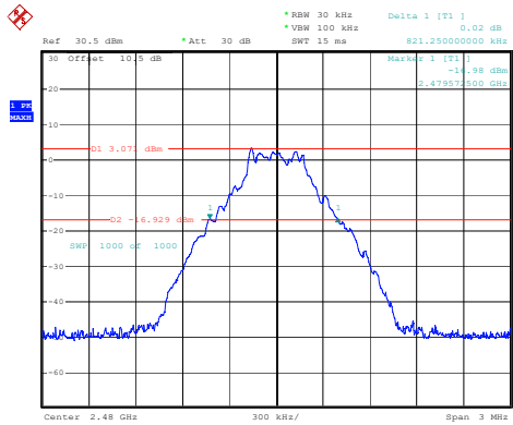
DH1_High 0.821MHz
