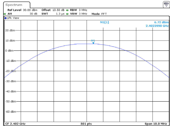
2DH1_Low 6.72dBm
