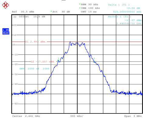
DH1_Middle 0.825MHz
