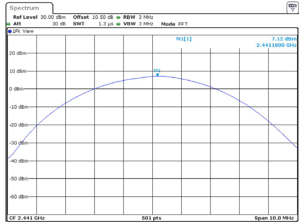
DH1_Middle 7.12dBm
