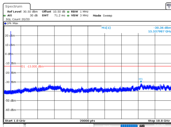
3MHz_Low_QPSK_1@0(1GHz~18.8GHz)
