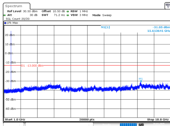
3MHz_Middle_QPSK_1@0(1GHz~18.8GHz)
