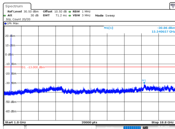
3MHz_Low_QPSK_15@0(1GHz~18.8GHz)
