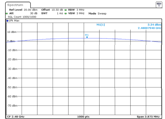
DH1_High 3.34dBm
