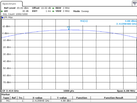
3DH1_Additional 4.88dBm
