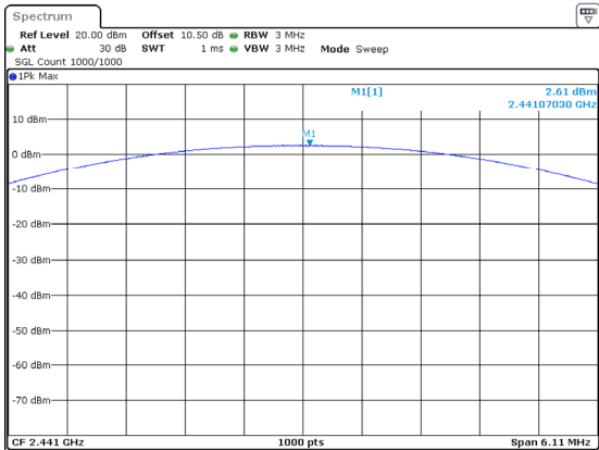
3DH1_Middle 2.61dBm
