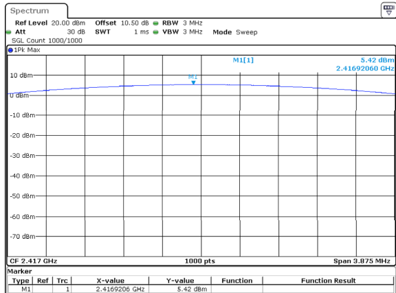
DH1_Additional 5.42dBm
