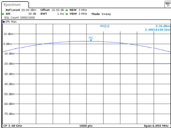
3DH1_High 2.76dBm
