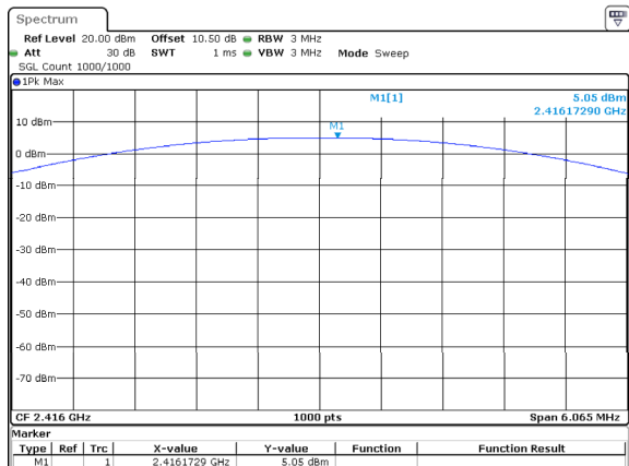
2DH1_Additional 5.05dBm
