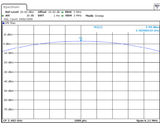
3DH1_Low 2.99dBm
