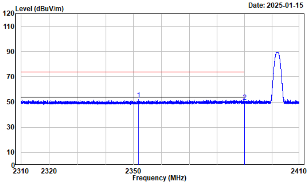
Left Band edge_Horizontal BLE1M-2402_2310-2390MHz
