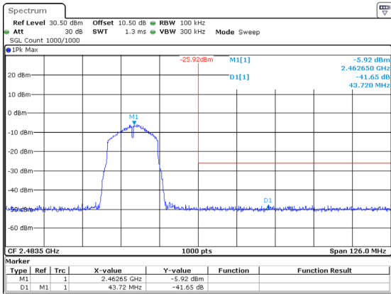
802.11g_2462MHz
