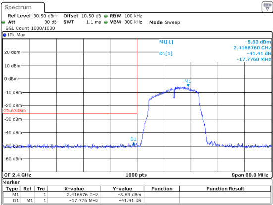
802.11g_2412MHz
