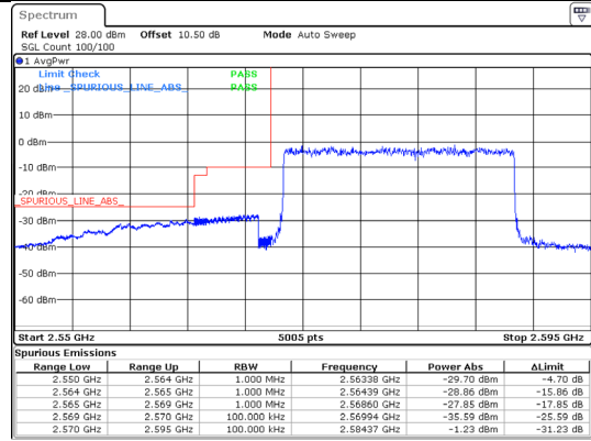
Band 38 20MHz/2580.0/Low QPSK 100@0
