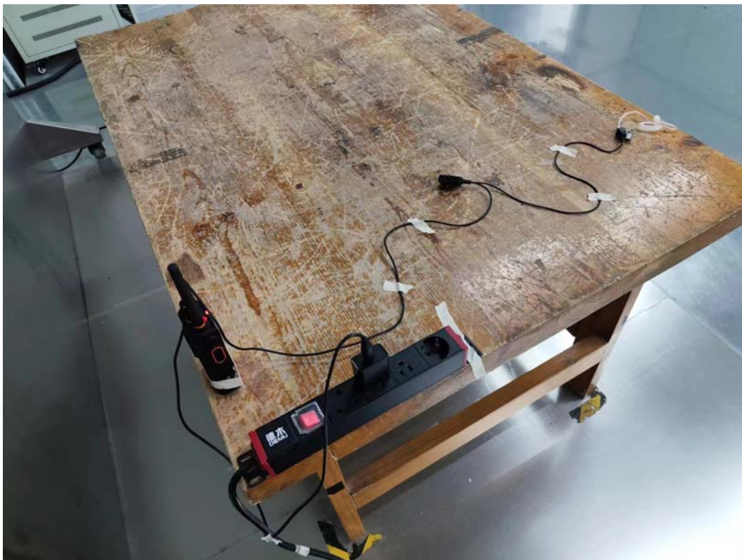
Conducted Emissions Side View Adapter + Small Hand Microphone
