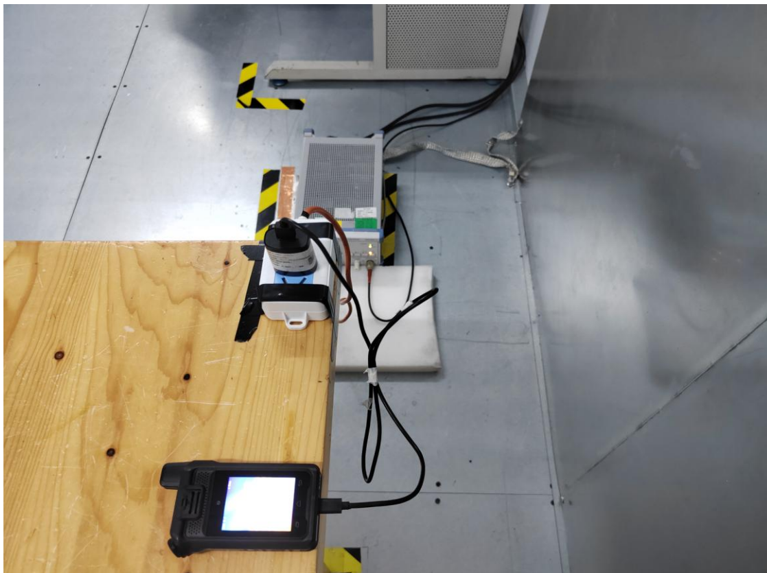
Photo of Power Line Conducted Emission Measurement-Side View-Without Card
