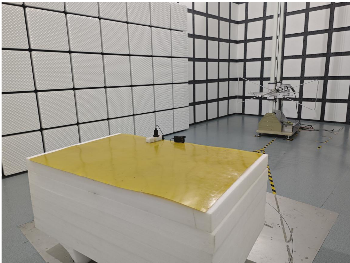
Radiated Spurious Emissions Test View (30MHz-1GHz)-Without Card
