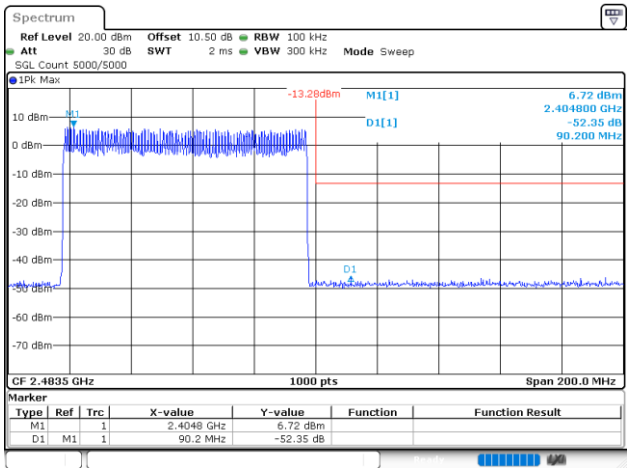
3DH5_Hopping_Upper
