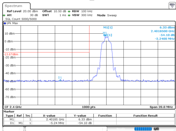
2DH5_Low
