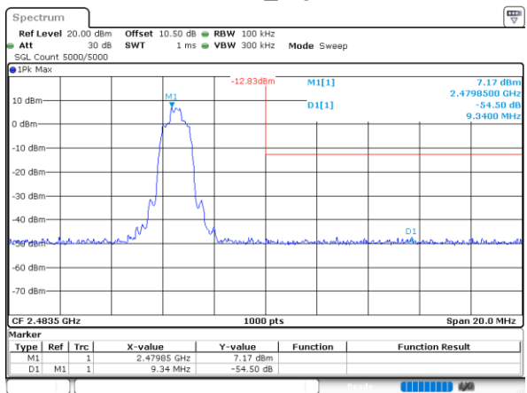
2DH5_High
