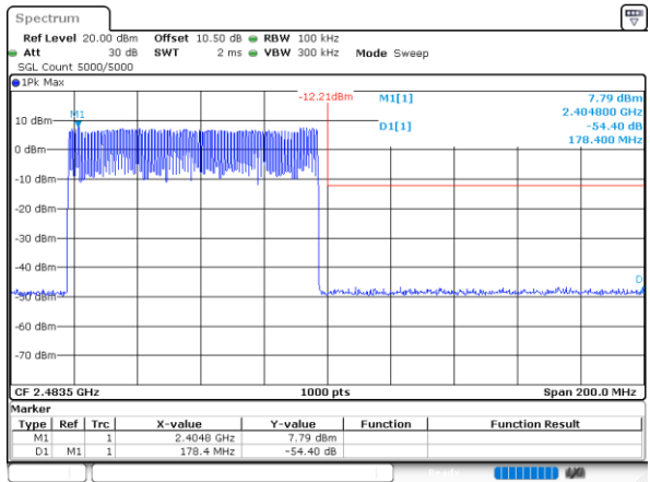
DH5_Hopping_Upper
