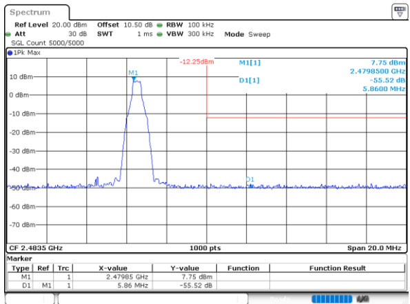
DH5_High
