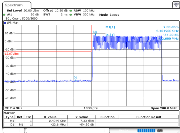
DH5_Hopping_Lower
